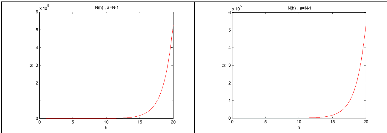
Figure 1. Minimal Grid Size for given Entropy Production for Automorphisms with (a) \det A=1 . (b) \det A=-1
