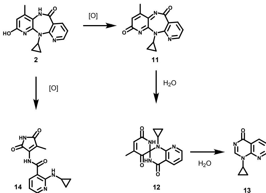
Scheme 3 Products obtained from 2-hydroxy-NVP oxidation with Frémy's salt.
