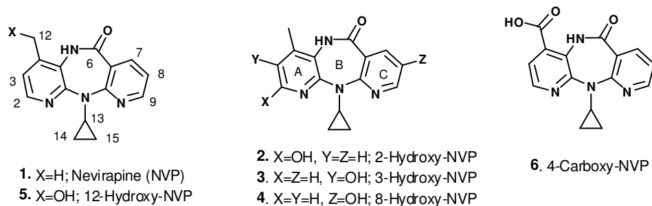
Scheme 1 Structures of Nevirapine ( 1 ) and its Phase I metabolites.
