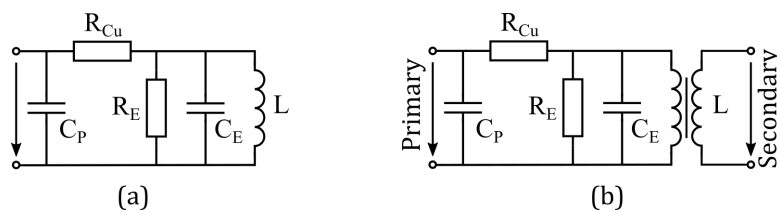
Figure 2: Equivalent circuit of (a) a single coil and (b) a coil pairing in conductive fluid, modeling the eddy current effect
