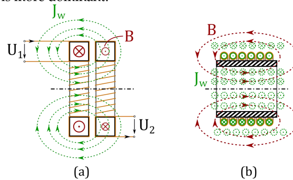
Figure 1: Schematic diagram of (a) a transformer type sensor and (b) an eddy current sensor. Green vectors display the current density, red the magnetic field strength. The sensors are surrounded by a conductive fluid.
