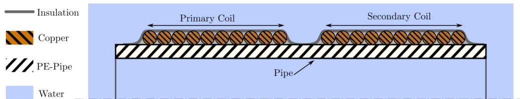
Figure 3: Schematic of the implemented eddy current sensor
