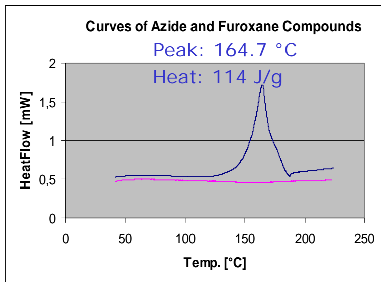
DSC diagram
