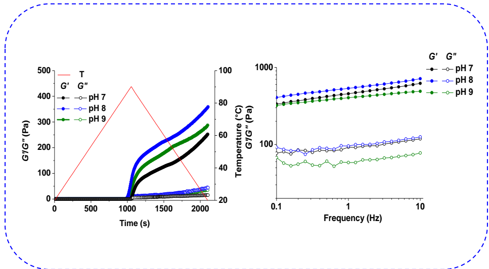
Rheological properties
