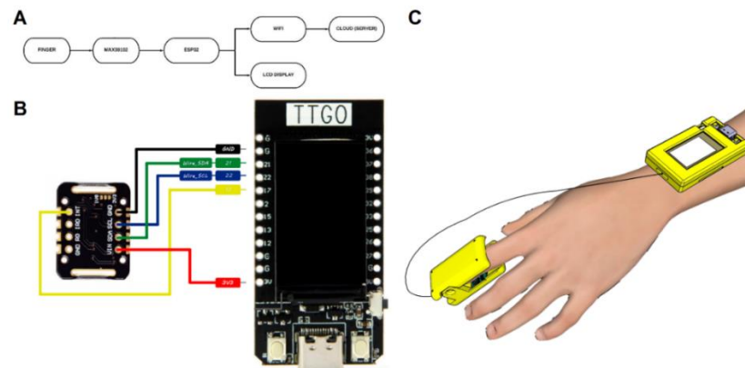
Figure 1. (A) Outline of the device functioning, wherein the signals from patient's finger is gathered by MAX30102 and transmitted to ESP32, which both displays the information on an LCD display, as well as send it to the cloud using the SoC IoT capabilities. (B) Circuit topology evidencing the use of MAX30102 and ESP32 SoC general-purpose input/output pins for communication between these two integrated circuits. (C) Rendering of the model used for the 3D printing of the device. ESP32 is housed in the wrist while the MAX30102 is in the finger of the user. The connections between MAX30102 and ESP32 were performed with 0.9 mm diameter jumper wires.
