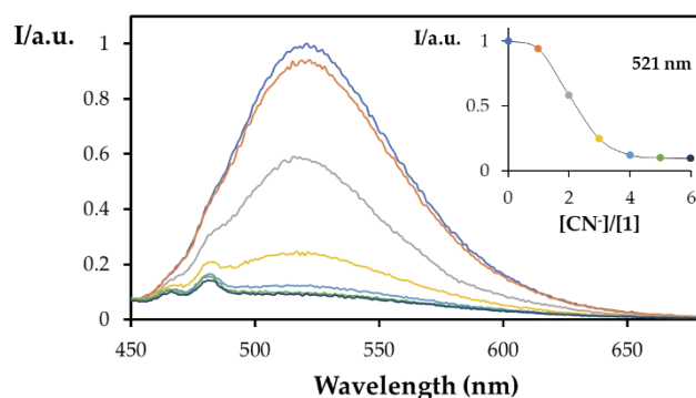
Figure 5. Spectrofluorimetric titration of dicyanovinyl derivative 1 with addition of increasing amounts of \text{CN}^- in ACN/ \text{H}_2\text{O} (8:2). The inset represents the normalized intensity at 521 nm ( [\text{1}] = 8.0 \times 10^{-6} M).
