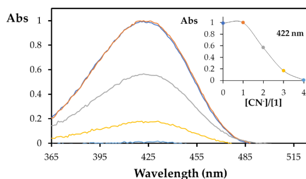
Figure 4. Spectrophotometric titration of dicyanovinyl derivative 1 with addition of increasing amounts of CN - in ACN/ H 2 O (8:2). The inset represents the normalized absorbance at 422 nm ( [1] = 8.0 \times 10^{-6} M).
