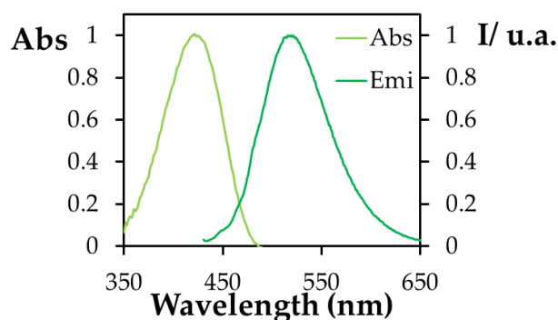
Figure 2. Normalized UV-visible absorption and emission spectra of the dicyanovinyl derivative 1 in ACN ( 1.0 \times 10^{-5} \text{M} , \lambda_{\text{exc}} = 421 \text{nm} ).
