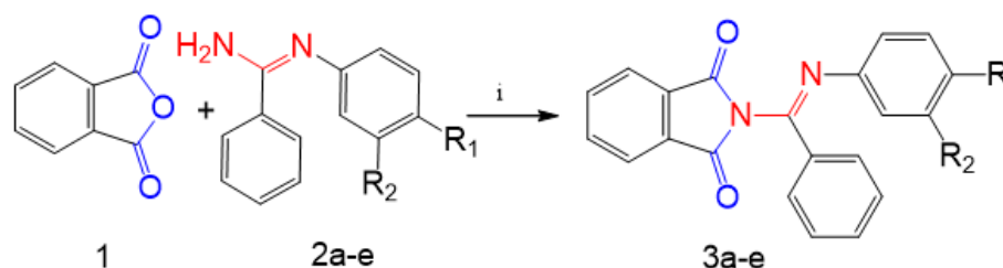
Figure 2. Scheme for the preparation of isoindoline-1,3-diones 3a-e ; i : benzene, \Delta , 4-7 hours.
