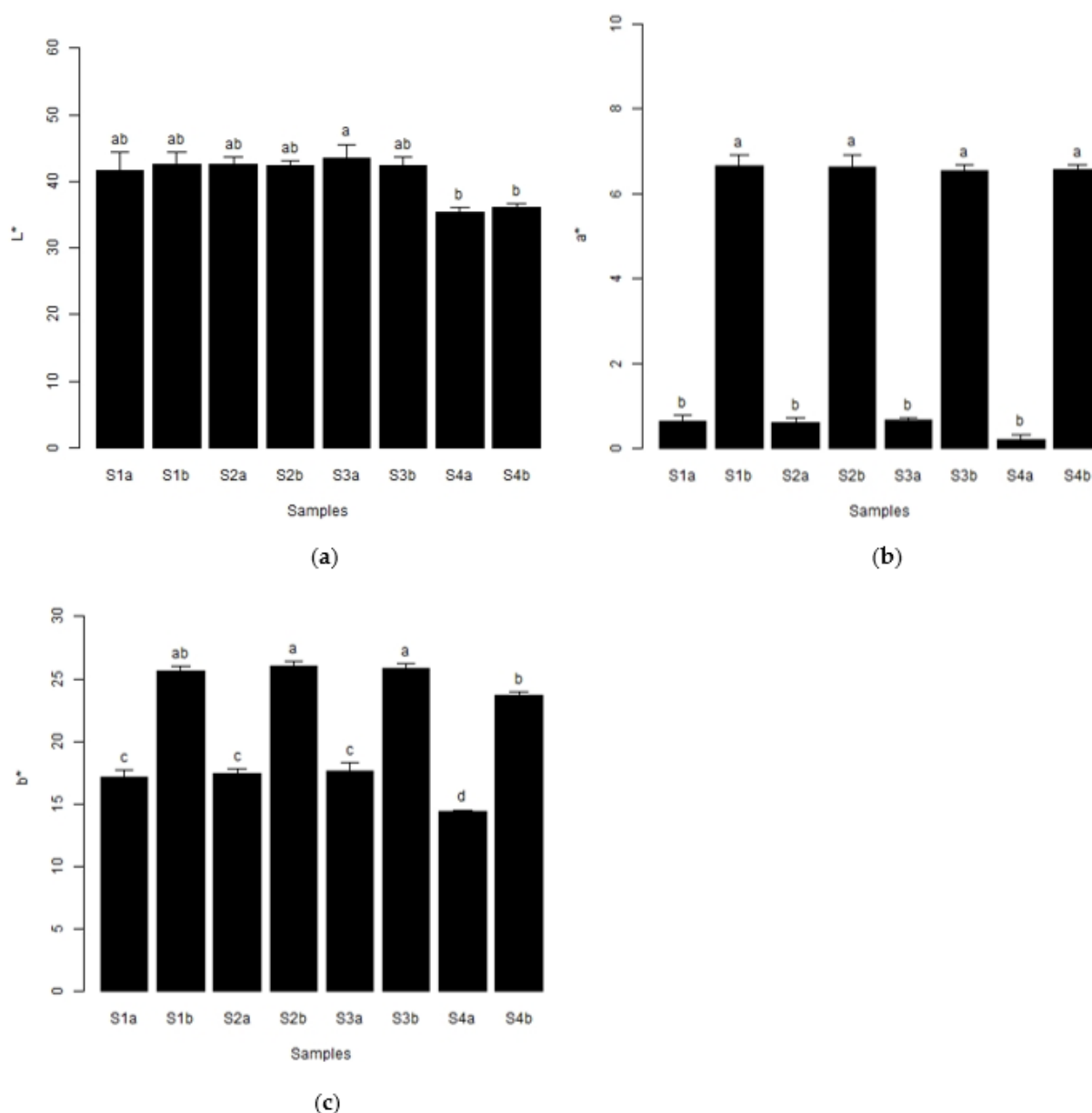
Figure 1. Colorimeter CIELab System with the color parameters ( n = 9 ): (a) L^* (lightness); (b) a^* (red-green transitions); and (c) b^* (yellow-blue transitions) of soil samples before (S1a, S2a, S3a and S4a) and after (S1b, S2b, S3b and S4b) performing organic matter content. Letters a, b, c, d indicate significant differences, of each parameter, considering different samples (statistical analysis using the single factor ANOVA test, p < 0.05 ).
