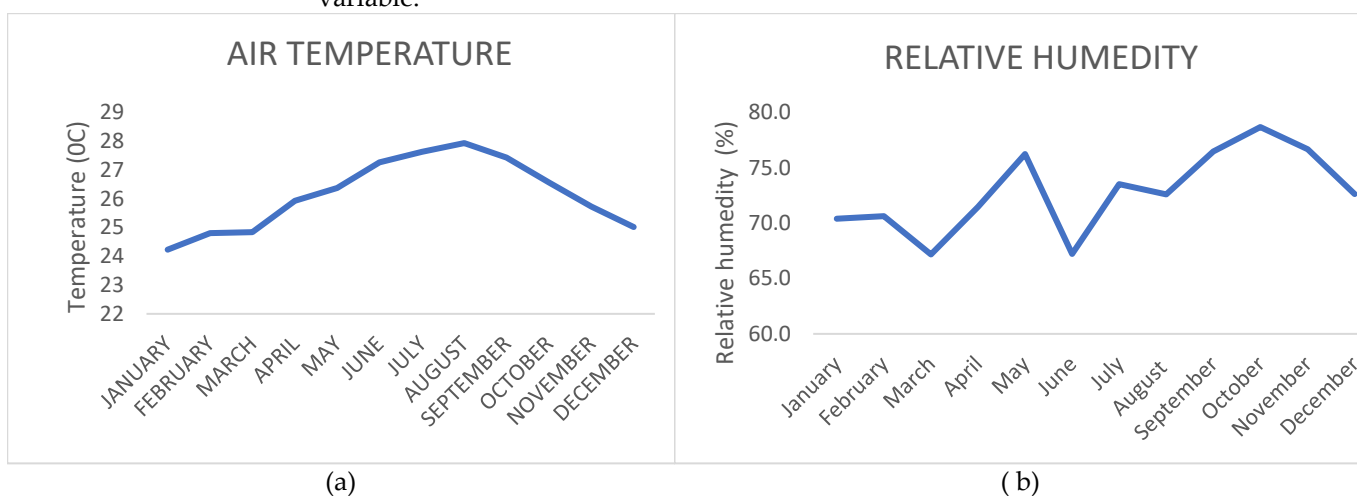
Figure 3. The behavior of (a) the mean air temperature and (b) relative humidity in MUCU in the period 2017-2021
