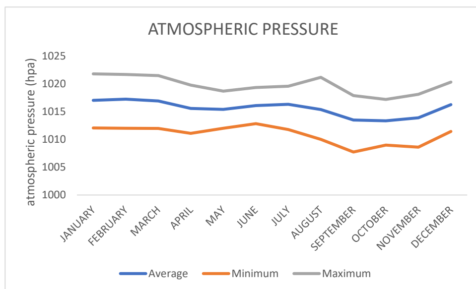
Figure 4. Annual behavior of the mean, minimum, and maximum atmospheric pressure in MUCU in the period 2017-2021.
