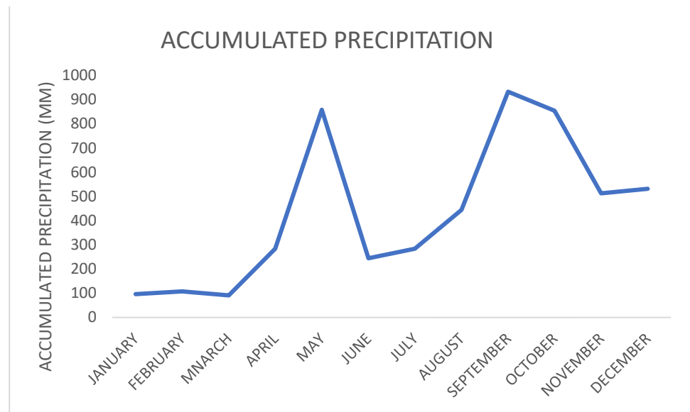
Figure 5. Behavior (a) monthly and (b) annual of the accumulated precipitation in MUCU in the period 2017-2021.
