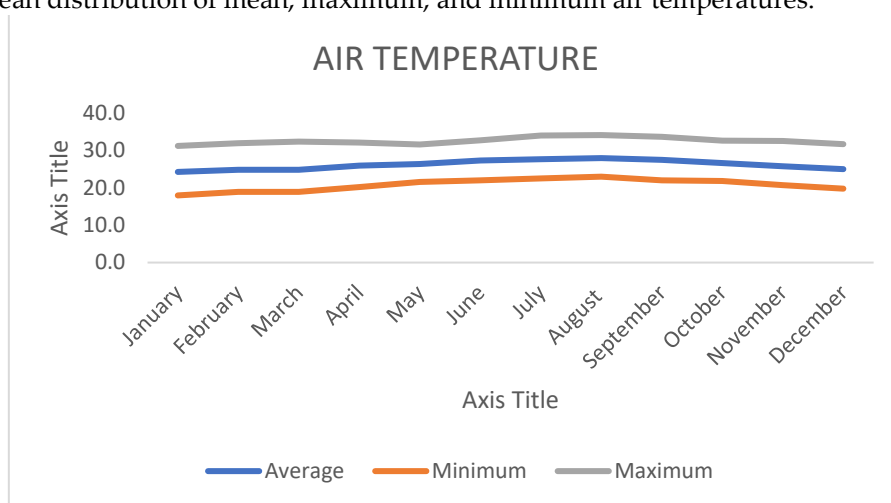
Figure 2. Mean distribution of mean, maximum, and minimum air temperatures
