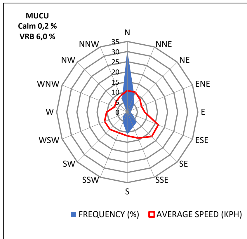
Figure 5. Rose of the winds corresponding to the period 2017-2021.
