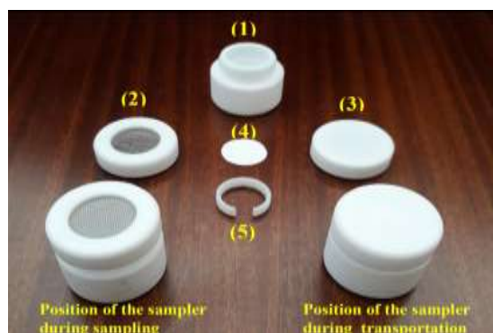
Figure 3. Parts of the tailor-made passive sampler [19].
