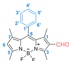
Figure 1. Structure of BODIPY derivative 2 .
