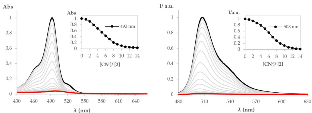
Figure 4. (a) Spectrophotometric and (b) spectrofluorimetric titration spectra of BODIPY derivative 2 upon addition of increasing quantities of CN^- (0–14 eq.) in acetonitrile. Inset: normalized absorbance and emission intensities at 492 nm and 508 nm, respectively, as a function of [CN^-]/[2] .
