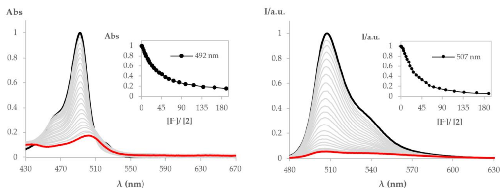
Figure 3. (a) Spectrophotometric and (b) spectrofluorimetric titration spectra of BODIPY derivative 2 upon addition of increasing quantities of F^- (0–190 eq.) in acetonitrile. Inset: normalized absorbance and emission intensities at 492 nm and 507 nm, respectively, as a function of [F^-]/[2] .
