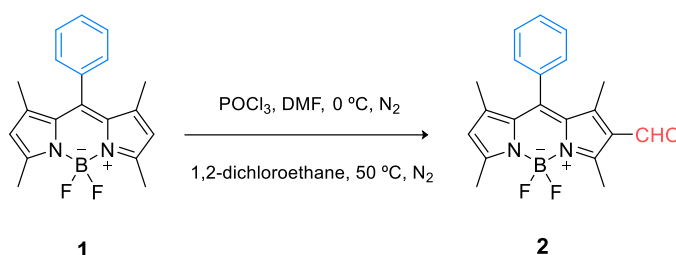
Scheme 1. Synthetic route for BODIPY derivative 2 .
