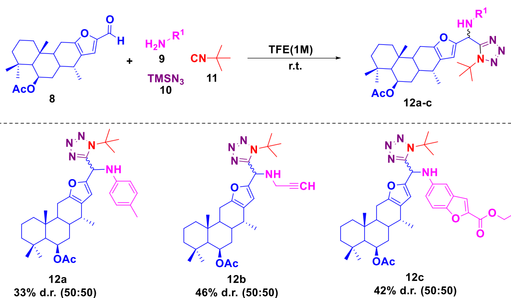
Scheme 1. Synthesis of 1,5-disubstituted tetrazoles-vouacapane 12a-c via Ugi-Azide multicomponent reaction.
