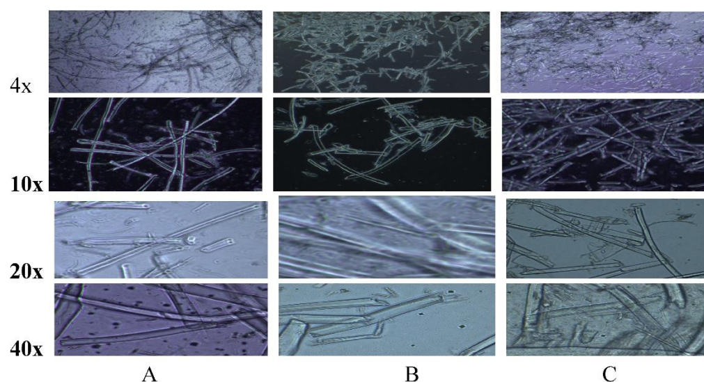
Figure 1. Microscopic images of the products of hydrolysis of the silkworm cocoon with NaOH solution at a concentration of 0.625 n, the duration of hydrolysis time of 90 min., magnification of the lens by 4, 10, 20, 40 times at temperatures: (A)—323 K; (B)—343 K; (C)—373 K.
