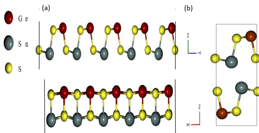
Figure 1. (a) Top and side monolayer's views, (b) the bulk structure of GeSnS2.
