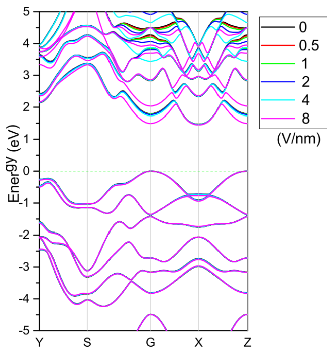
Figure 3. The effect of electric field on the band structure of monolayer GeSnS2.
