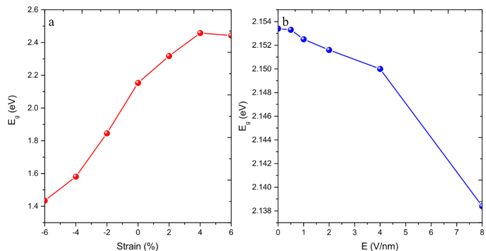
Figure 3. The variation of band gap energy with (a) strain and (b) electric field.
