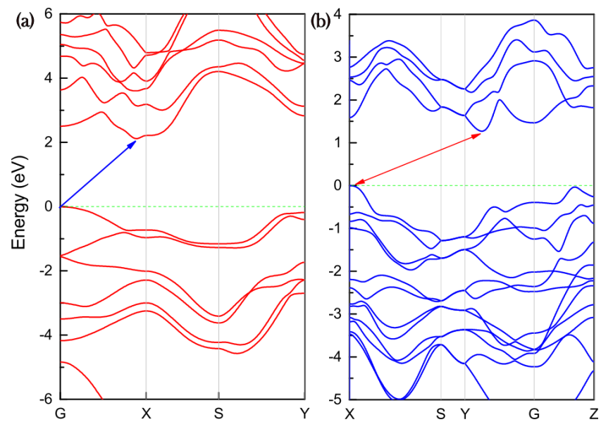
Figure 2. The band structure of (a) monolayer, (b) the bulk of GeSnS2.
