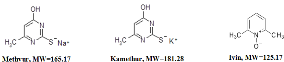
Figure 1. Chemical structure and relative molecular weight of plant growth regulators Methyur, Kamethur and Ivin.
