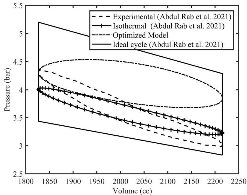
Figure 1. Comparison of the Optimized Model with another thermodynamic model.
