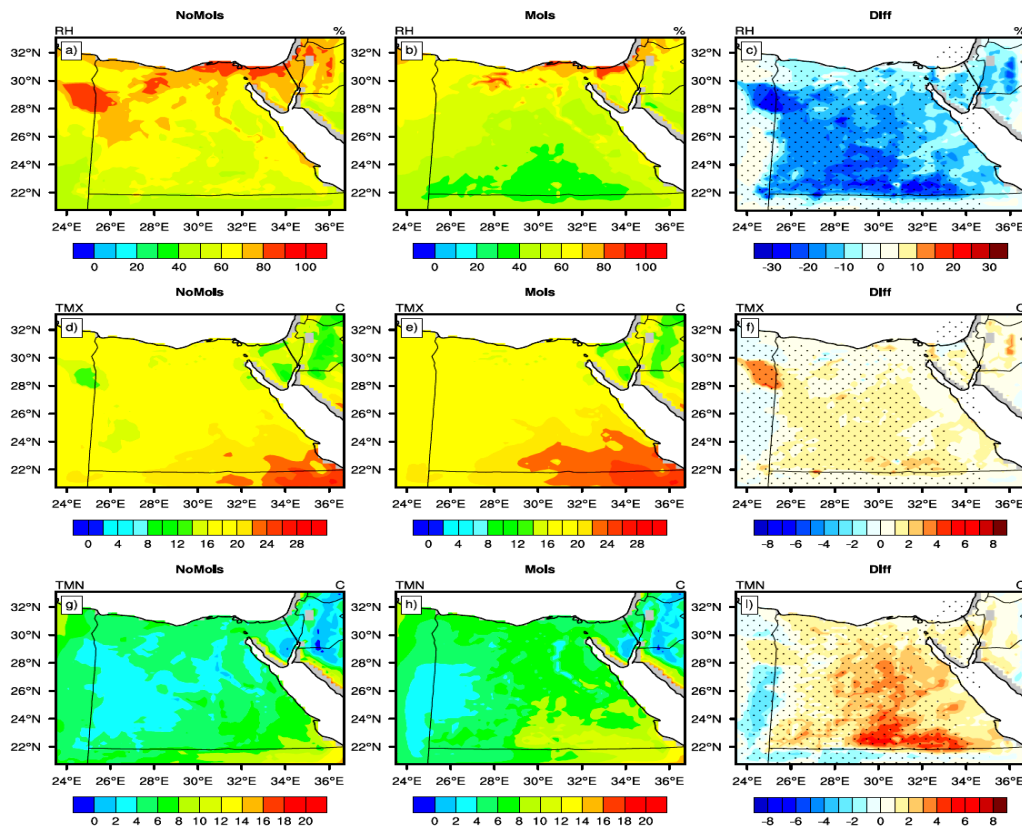
Figure 4. The figure shows the comparison between NoMols and MoIs for the variables: 1—near surface relative humidity (RH; (a–c)), 2—near surface maximum air temperature (TMX; (d–f)) and 3—near surface minimum air temperature (TMN; (g–i)).
