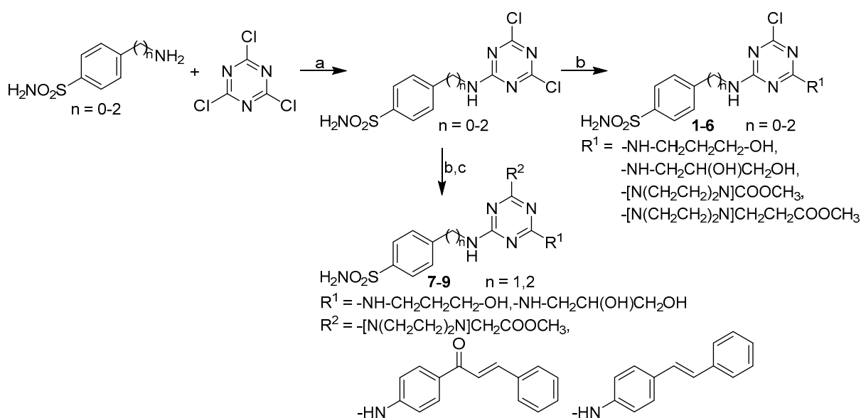
Scheme 1. Synthesis of target compounds 1–9. Reagents and conditions: (a) acetone, 0–5 ^{\circ}\text{C} [39]; (b) suitable amine derivative (1 eq.), DMF, K 2 CO 3 , 35 ^{\circ}\text{C} ; (c) suitable amine derivative (1 eq.), DMF, K 2 CO 3 , 100 ^{\circ}\text{C} [35–38].
