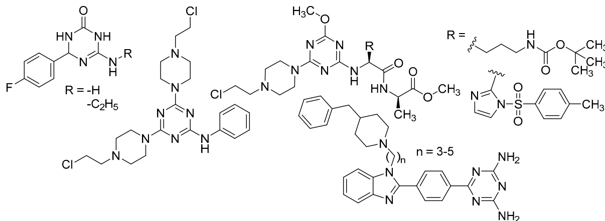
Figure 1. Selected recently published structures of 1,3,5-triazine-based BACE1 inhibitors [17–19].
