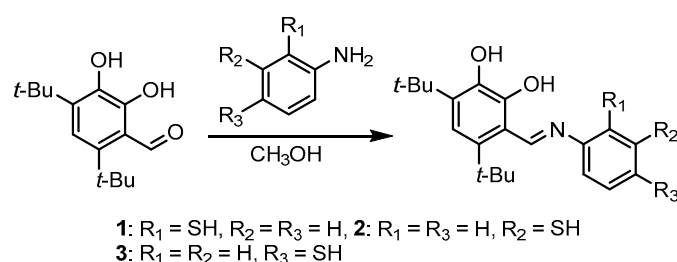
Figure 1. Synthetic scheme for the compounds 1–3.
