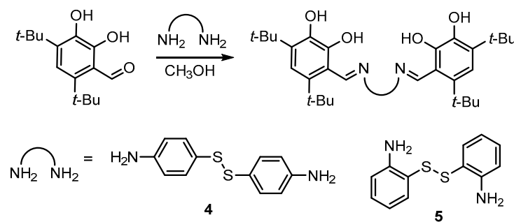
Figure 2. Synthetic scheme for the compounds 4 and 5.
