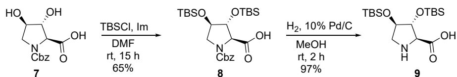
Scheme 3. Synthesis of proline 9 .
