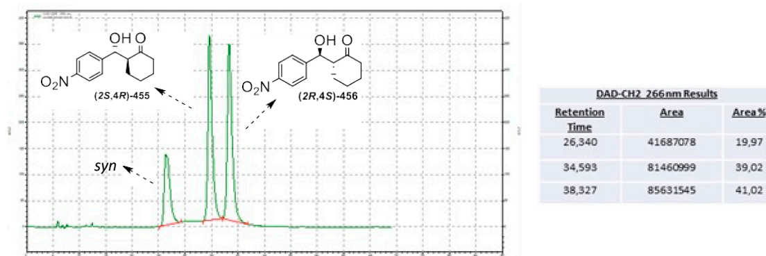
Figure 2. Chromatogram of racemic mixtures of the aldols 10-13 .
