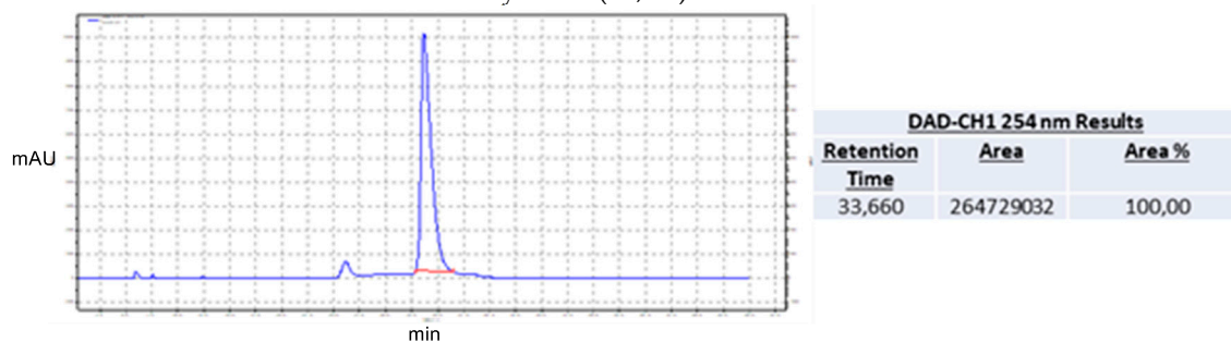
Figure 3. Chromatogram of the aldol mixture of the standard reaction with catalyst 9 .
