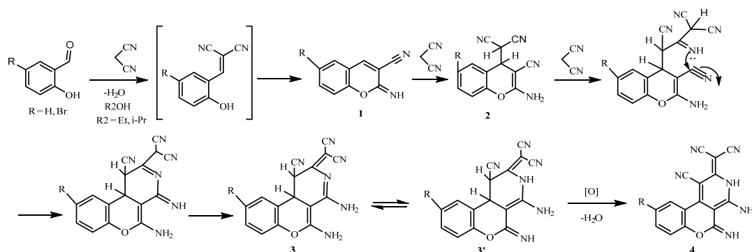
Scheme 2. Proposed mechanism for the reaction between salicylaldehyde and malononitrile for the synthesis of 2-amino-4H-chromene.
