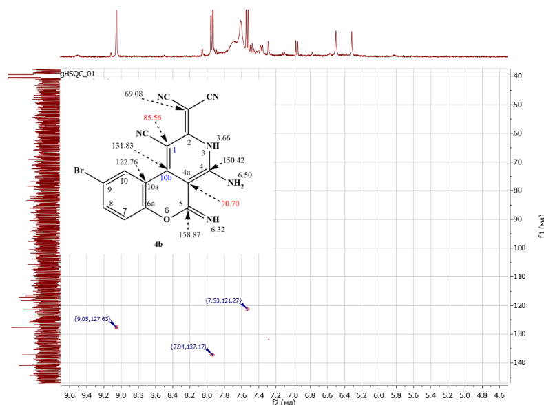
Figure 1. NMR HSQC ^1\text{H}/^{13}\text{C} spectrum and main correlations in the NMR HSQC ^1\text{H}/^{13}\text{C} and HMBC ^1\text{H}/^{13}\text{C} spectrum of 4b .
