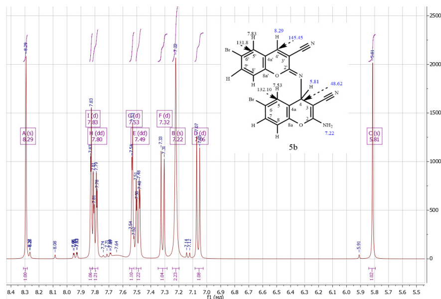
Figure 2. ^1H NMR spectrum of compound 5b .
