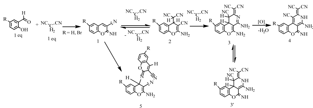
Scheme 1. Reactions between salicylaldehyde and malononitrile for the synthesis of imino(amino)cyanochromenes derivatives.
