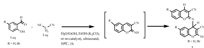
Scheme 3. The synthesis of 2-iminochromene 1 dimers-2-amino-6-R-4-((6-R-3-cyano-2H-chromen-2-ylidene)amino)-4H-chromene-3-carbonitriles 5a,b .
