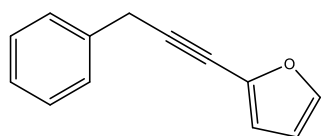
Figure 1. Carlina oxide.
