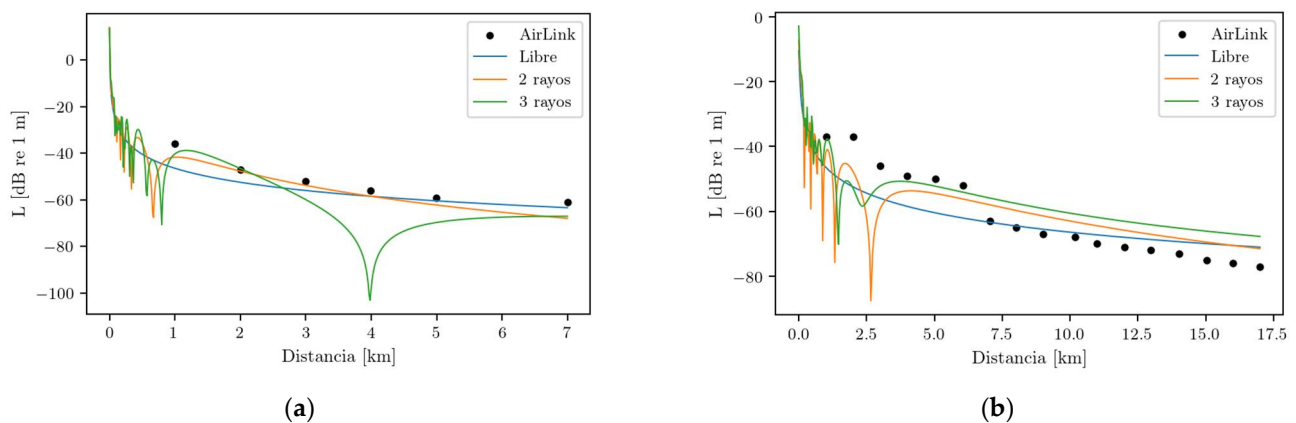
Figure 5. Comparison of Results Between Propagation Loss Models and AirLink Software for: (a) First test; (b) Second test.
