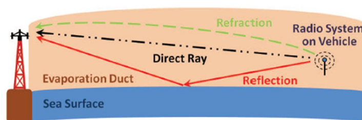
Figure 2. Ray tracing corresponding to the different number of ray model.
