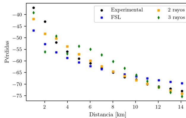
Figure 6. Comparison between experimental data (black circles) and those provided by the analytical models (remaining data).
