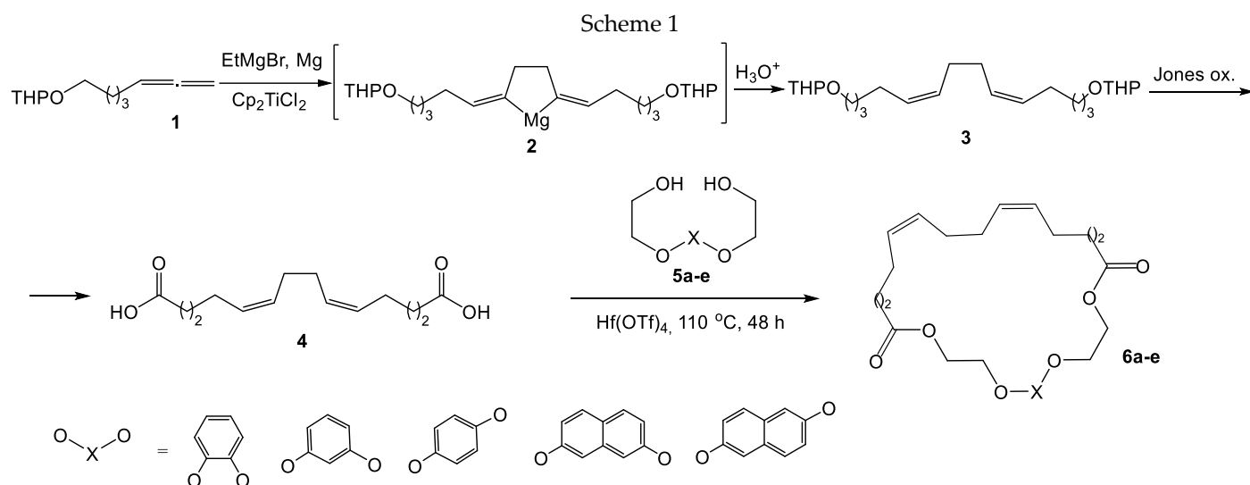
Scheme 1. Synthesis of aromatic polyether macrodiolides.
