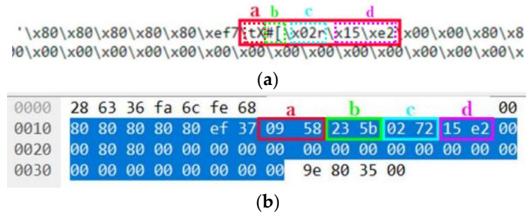
Figure 2. Raw data attributes from a PROFINET data packet: a = Current Speed, b = Electric Current, c = Motor Torque, d = Power Factor.
