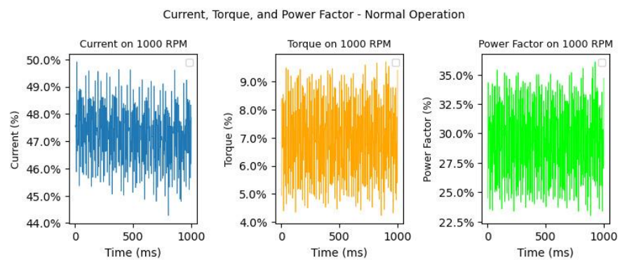
Figure 3. Behavior of the variables during 1 s of sampling in normal condition at 1000 RPM.
