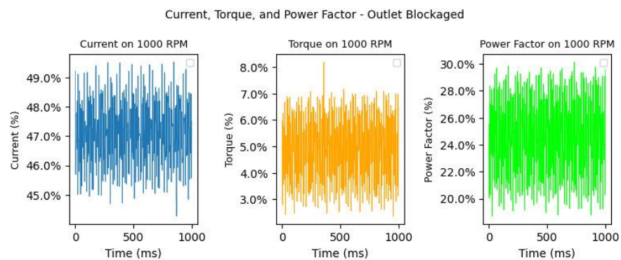
Figure 5. Behavior of the variables during 1 s of sampling with outlet blocked at 1000 RPM.
