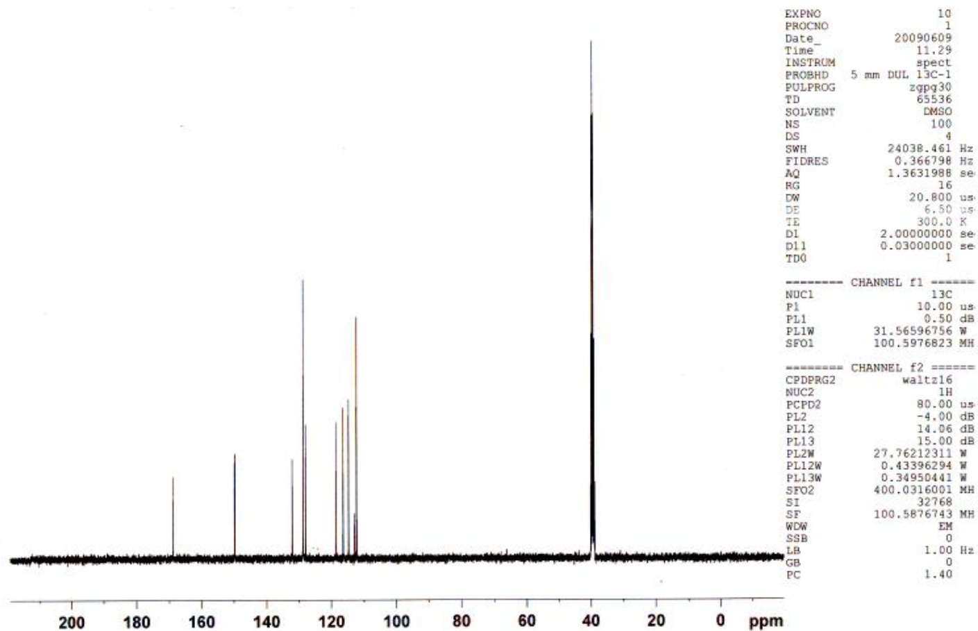
^{13}\text{C} -NMR spectra of N-(2-Amino-benzoyl)-N'-phenyl hydrazine
