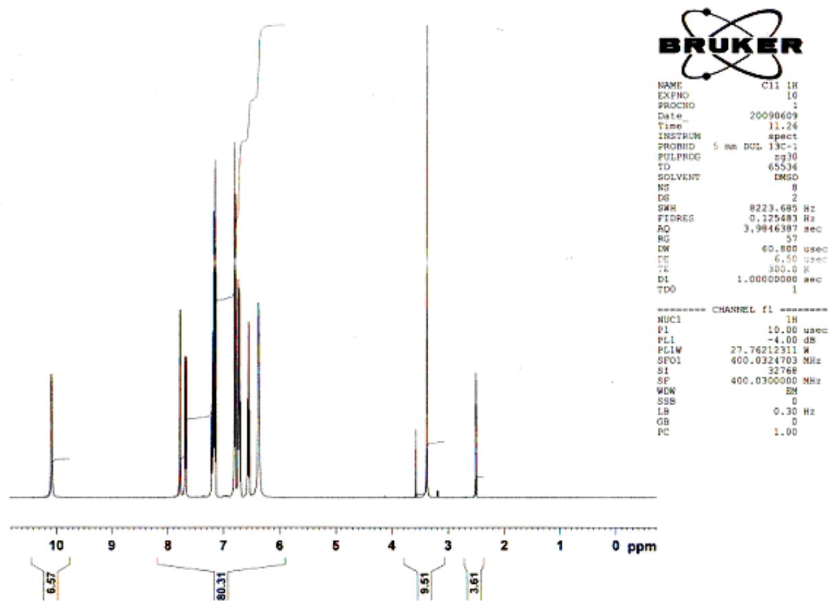
^1\text{H-NMR} spectra of N-(2-Amino-benzoyl)-N'-phenyl hydrazine
