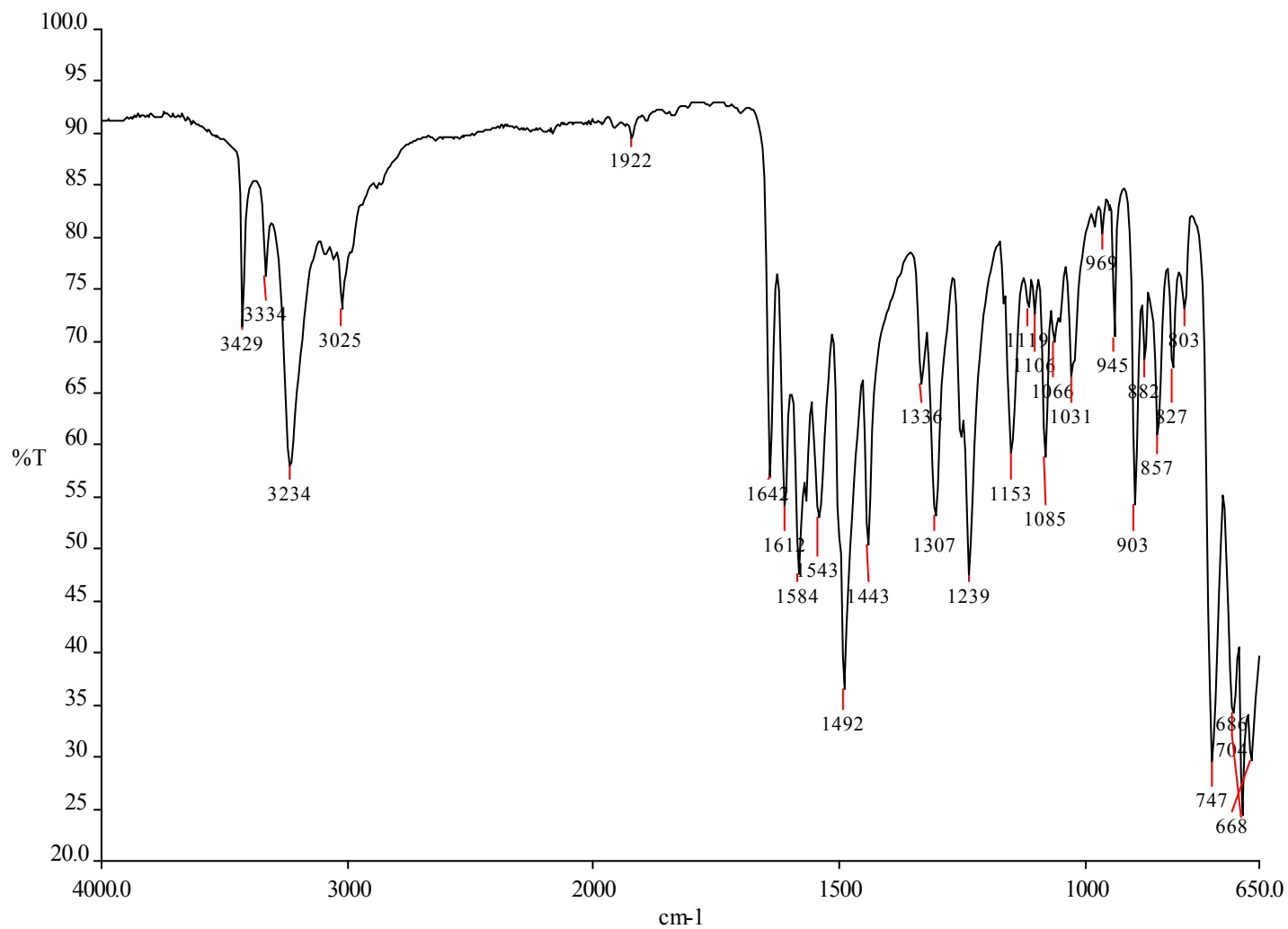
IR spectra of N-(2-Amino-benzoyl)-N'-phenyl hydrazine
