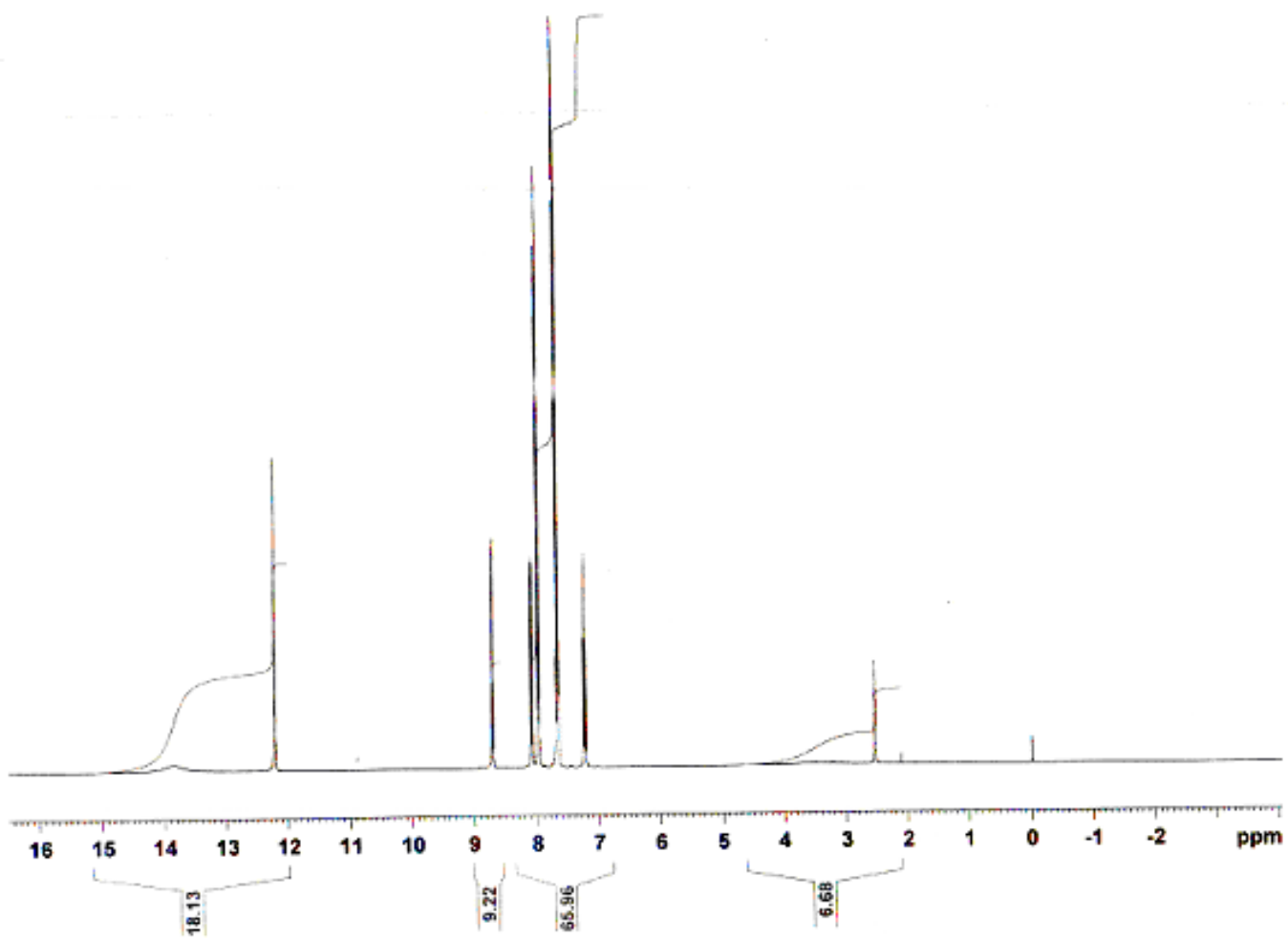
^1\text{H-NMR} spectra of N -(4-Chlorobenzoyl)-Anthranilic Acid
