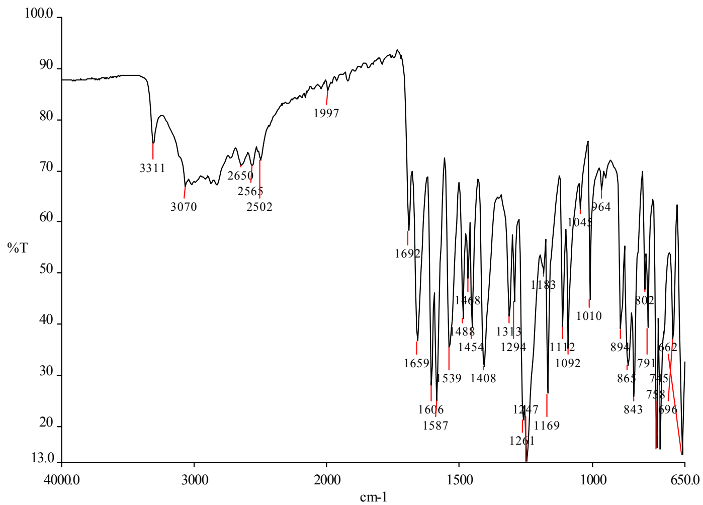
IR spectra of N -(4-Chlorobenzoyl)-Anthranilic Acid
