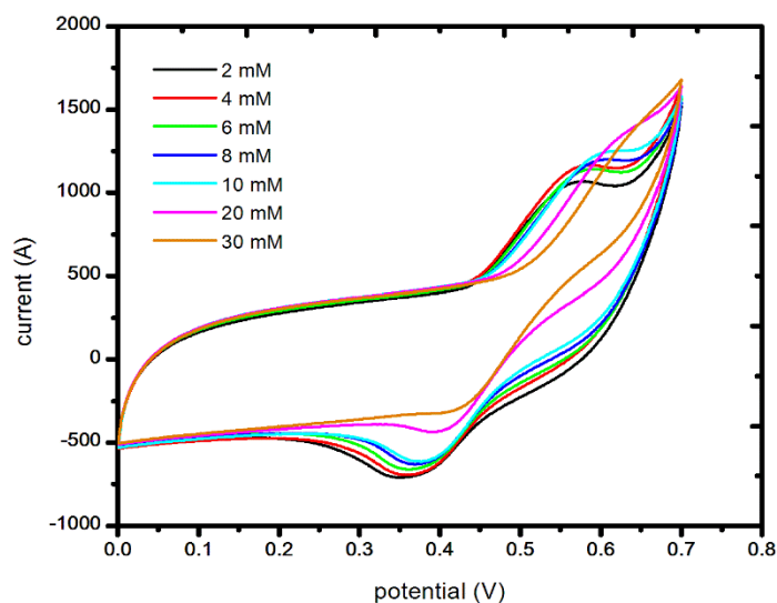
Fig 4. peak currents in Ni/CS/CNTs electrode depend on concentration of glucose
