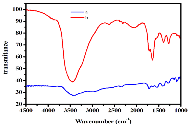
Fig. 1. FTIR spectra of the MWCNT-COOH (a) and CS-MWCNT (b)
