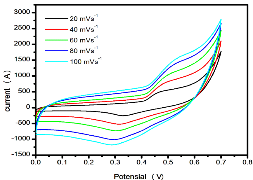
Fig3: cyclic voltammetry of of Ni/CS/CNTs nanocomposite film electrode in NaOH 0.1M at different scan rates
