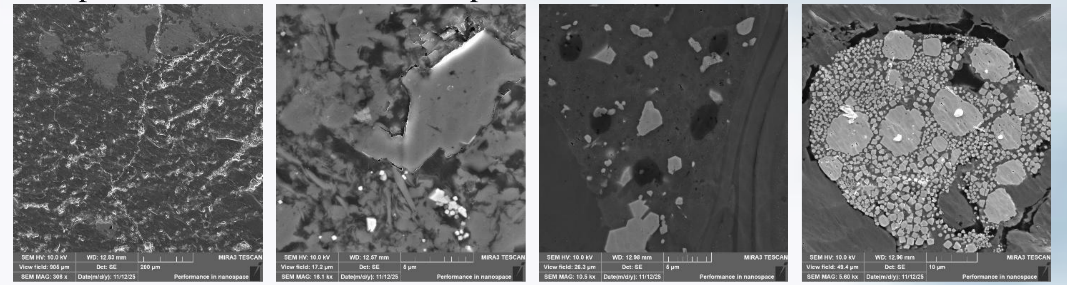
Fig.4 High-resolution SEM images of the Longtan Formation shale samples
