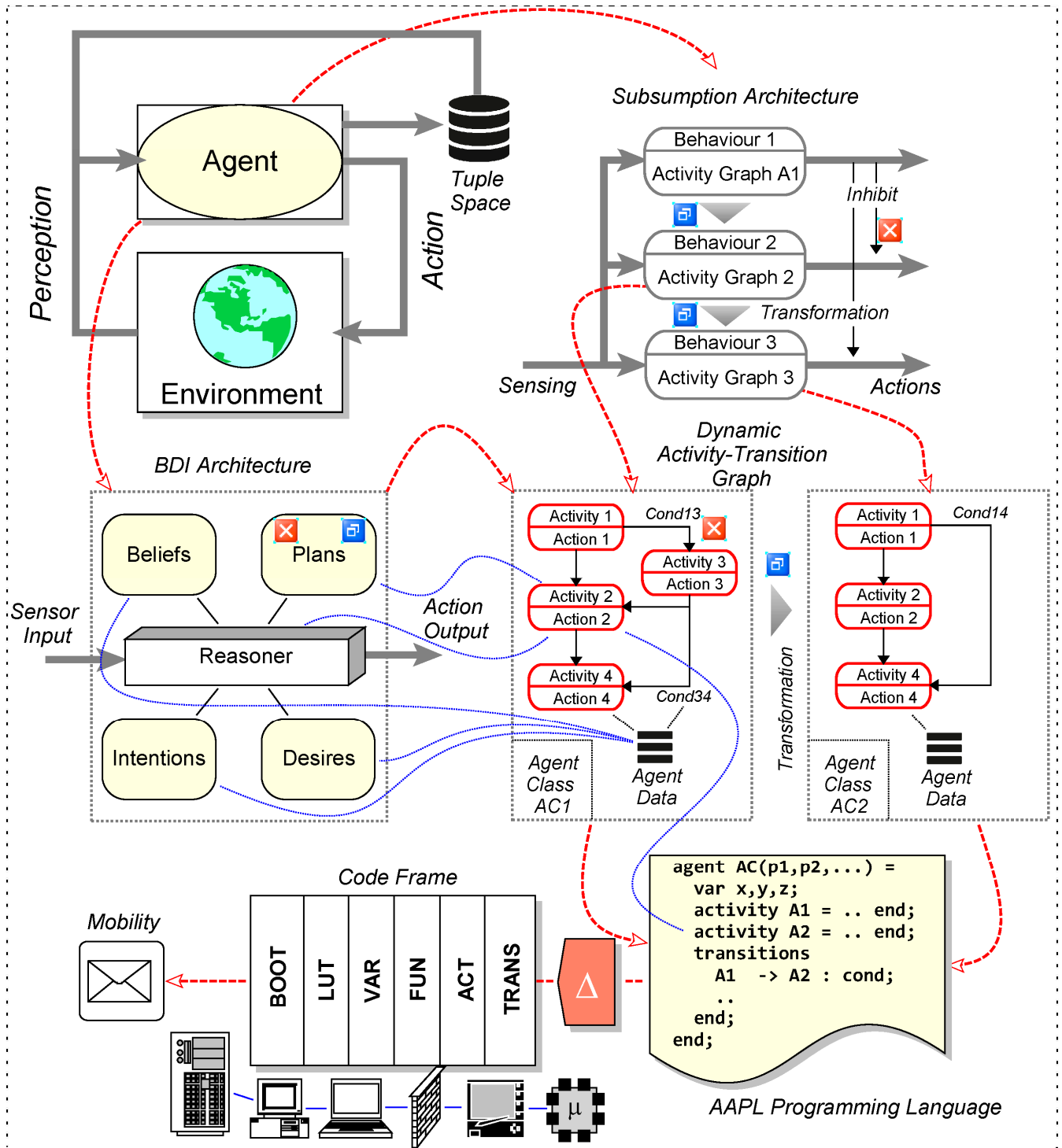
Figure 1. Agent Models: (Left, top) Basic Agent Model, (Right, top) Subsumption Architecture composed of different behaviour, (Right, middle) Reconfigurable (Dynamic) Activity-Transition Graphs (DATG) used in this work, (Left, middle) Relation to the Belief-Desire-Intention (BDI) Architecture, (Bottom) Programming model and code frame.
