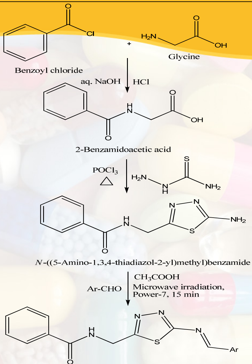
( E )- N -((5-(Substituted methyleneamino)-1,3,4-thiadiazol-2-yl)methyl)benzamide
