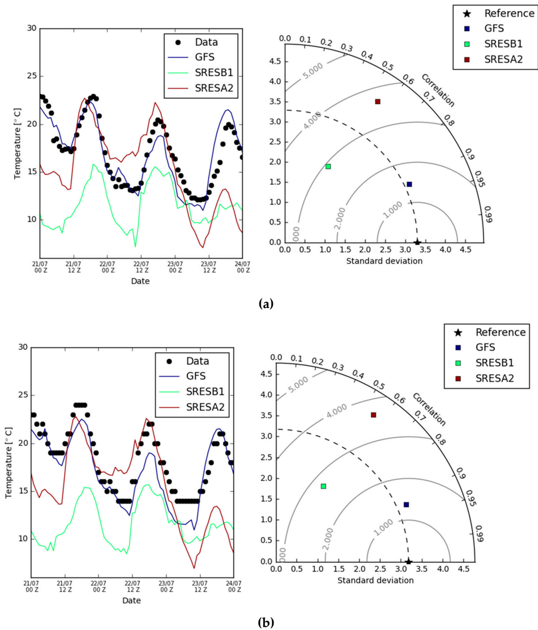
Figure 4. Evolution of temperature (left column) and Taylor diagram (right column) for (a) SIMEPAR and (b) Londrina Airport METAR data stations. Blue line is the simulation with GFS as input and boundary conditions, green line is the simulation with B1 scenario and red line is the simulation with A2 scenario. Both are output from CCSM3 model.
