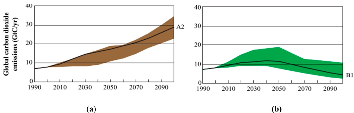
Figure 1. Future projection of global carbon dioxide emission for the (a) A2 and (b) B1 scenarios from SRES. From Nakicenovic et al (2000) [5].
