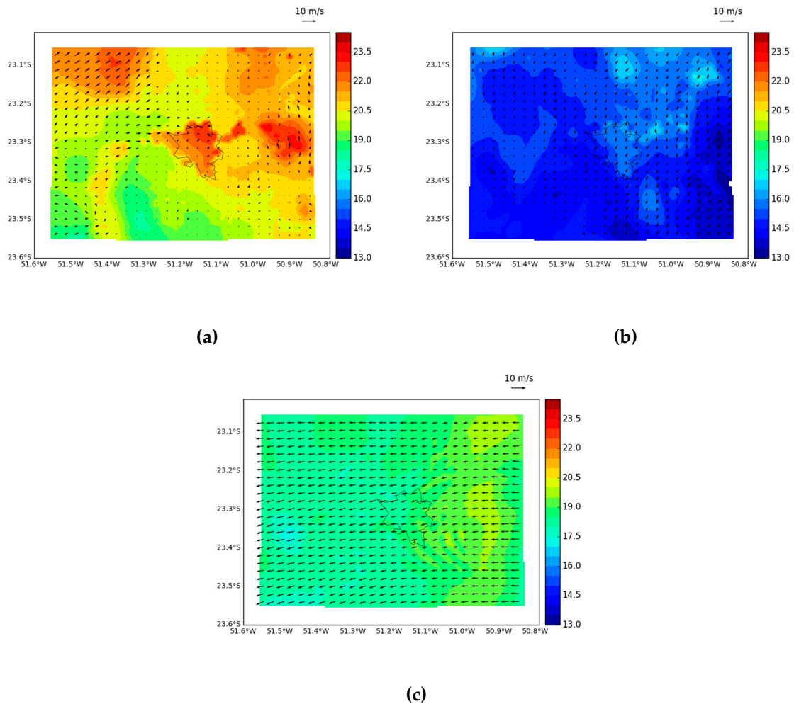
Figure 6. Air temperature at 2 m (in °C) for 18 Z at 22th July of 2015 for simulation with (a) SRESA2, (b) SRESB1 and (c) GFS simulations. Black arrow is the wind velocity intensity at 10 m.
