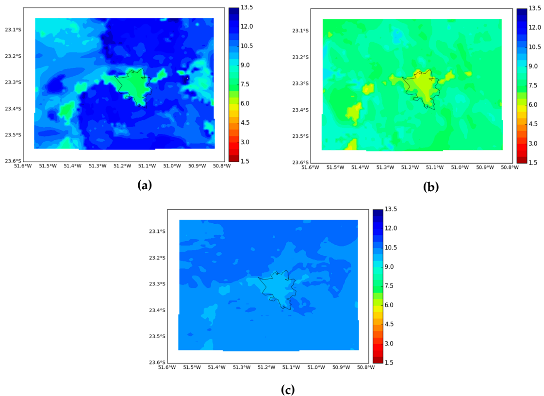
Figure 7. Specific humidity at 2 m (in g/kg) for 18 Z at 22 th July of 2015 for simulation with (a) GFS, (b) SRESB1 and (c) SRESA2 simulations.
