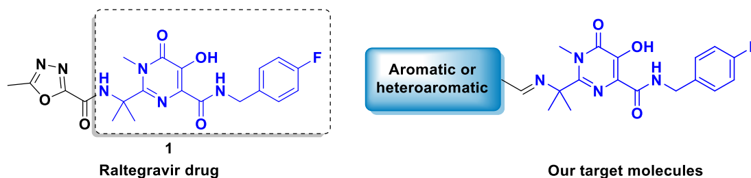
Figure 1. Raltegravir drug 1 and target molecules (Imines-Ralt)
