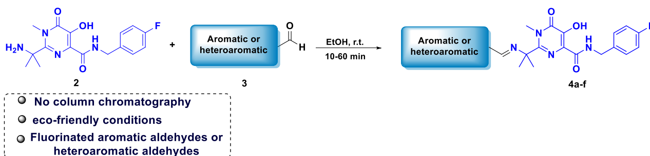
Scheme 1. General synthetic scheme for the synthesis of imines-Ralt 4a-f .
