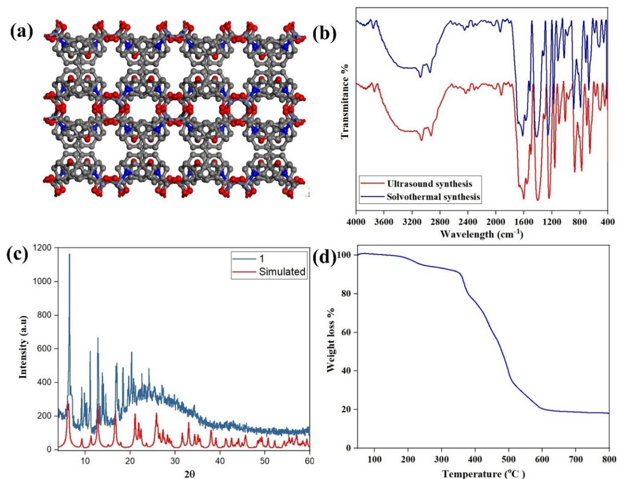
Figure 1. (a) Crystal structure of the 3D framework [Zn 2 (oba) 2 (bpy)] ( 1 ), showing the 1D channels running along the a axis (The disordered guest molecules are omitted for clarity). (b) FT-IR spectra of sonochemical (red) and solvothermal (blue) synthesized 1 . (c) PXRD of as-synthesized (blue) and simulated (red) [Zn 2 (oba) 2 (bpy)] ( 1 ). (d) TGA of activated [Zn 2 (oba) 2 (bpy)] ( 1 ).
