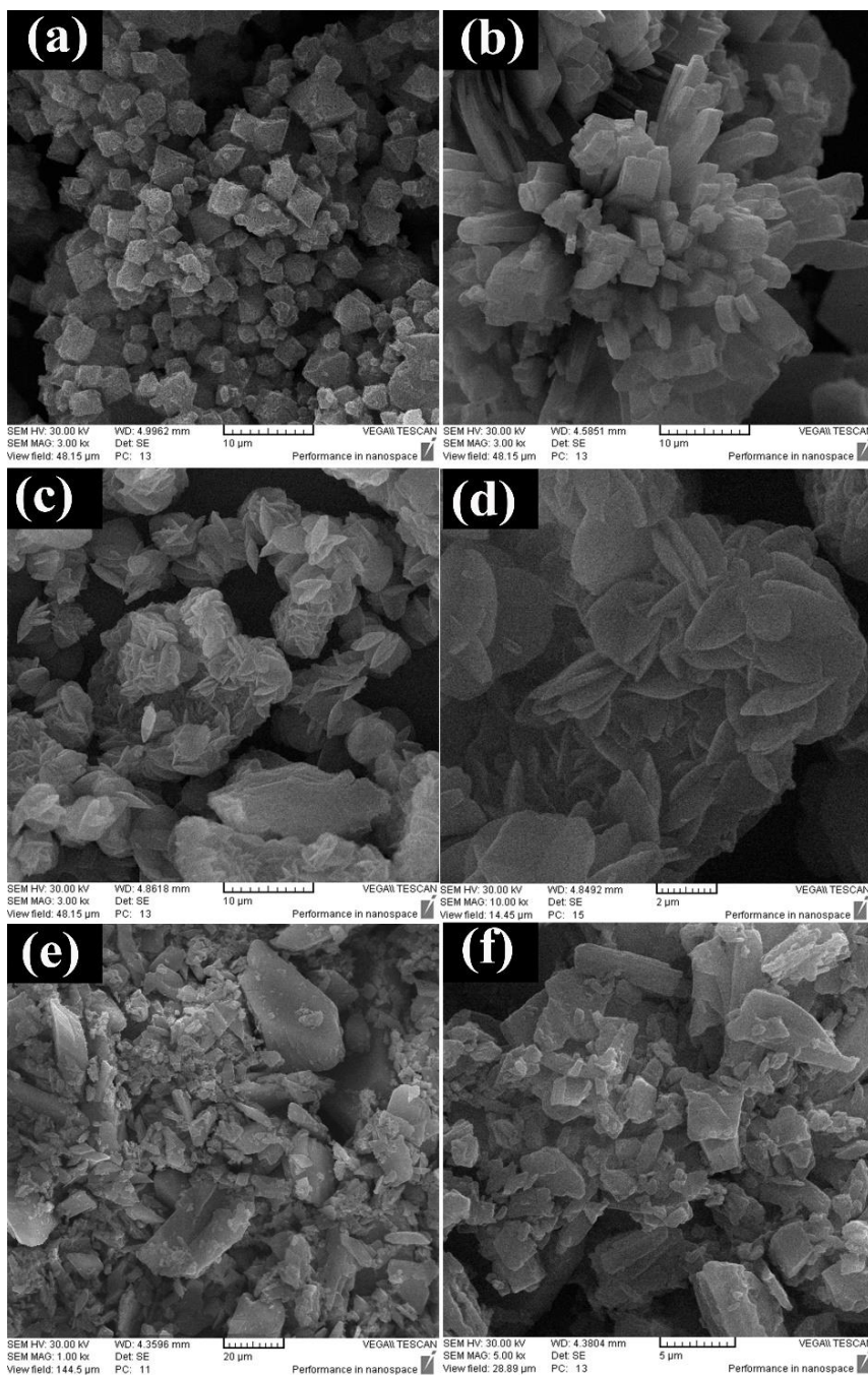
Figure 2. SEM images of [Zn_2(oba)_2(bpy)] ( 1 ) nanostructures prepared by US generator power of 50W at 1 h irradiation time in different concentration of initial reagents (a) 0.01 M, (b) 0.02 M and (c, d) 0.04 M. (e, f) SEM image of 1 bulk powder formed via solvothermal reaction without ultrasonic irradiation.
