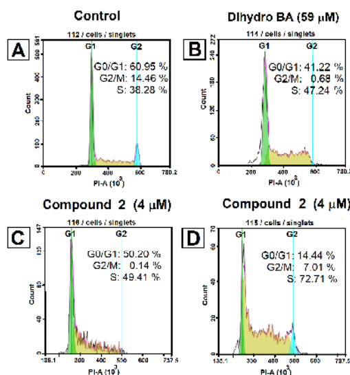
Figure 4. Cell cycle analysis in Jurkat cells. Jurkat cells were treated with tested compound 2 at the \text{IC}_{50} concentration for 24–48 h and dihydrobetulinic acid for 48 h. The cells were trypsinized, harvested and washed three times with ice-PBS for PI-stained DNA content detected by flow cytometry. The experiments were performed three times, and the results of the representative experiments are shown. The first cytogram represents an untreated cell sample (A); after incubation with dihydrobetulinic acid for 48 h (B); after incubation with compound 2 for 24 h (C) and for 48 h (D).
