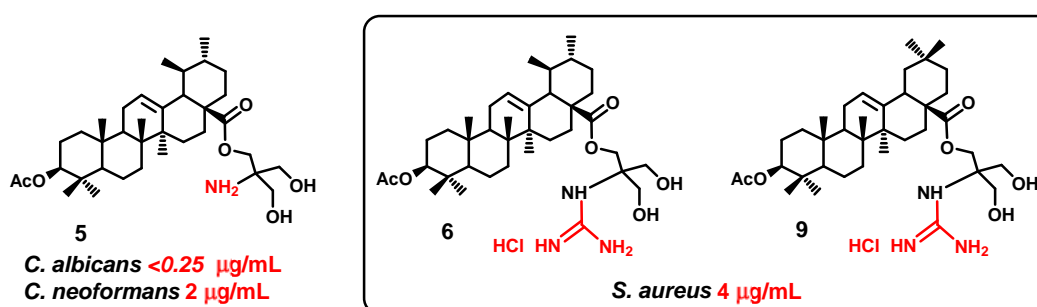
Figure 5. Structures of lead compounds 5 , 6 and 9 .
