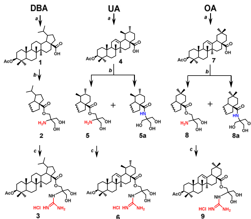
Scheme 1. Synthesis of compounds 2 , 3 , 5 , 5a , 6 , 8 , 8a and 9 . Reagents and conditions: (a) AcCl, THF, Py, DMAP, r.t.; (b) 1. (COCl) 2 , CH 2 Cl 2 ; 2. tris(hydroxymethyl)aminomethane, DMAP, Py, CH 2 Cl 2 , r.t.; (c) 1H-Pyrazole-1-carboxamide hydrochloride, DIPEA, DMF, r.t., 24 h.
