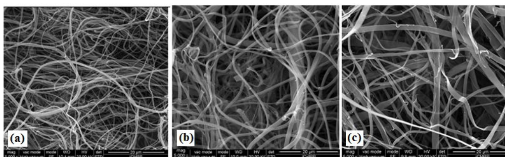
Figure 3. SEM images of PSFQ fibers obtained in various mixing ratios of solvents: 75DMF/25 2-MOEt (a), 50DMF/50 2-MOEt (b), 25DMF/75 2-MOEt 2-MOEt (c) at 40% concentration for 50 \mu\text{m} scan area and magnification of 2000x.
