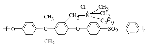
Scheme I. Chemical structure of the monomer units of the polysulfone with quaternary groups (PSFQ).
