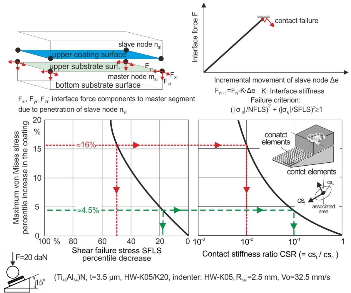
Figure 6. Relationship between contact stiffness ratio and shear failure stress percentile decrease.
