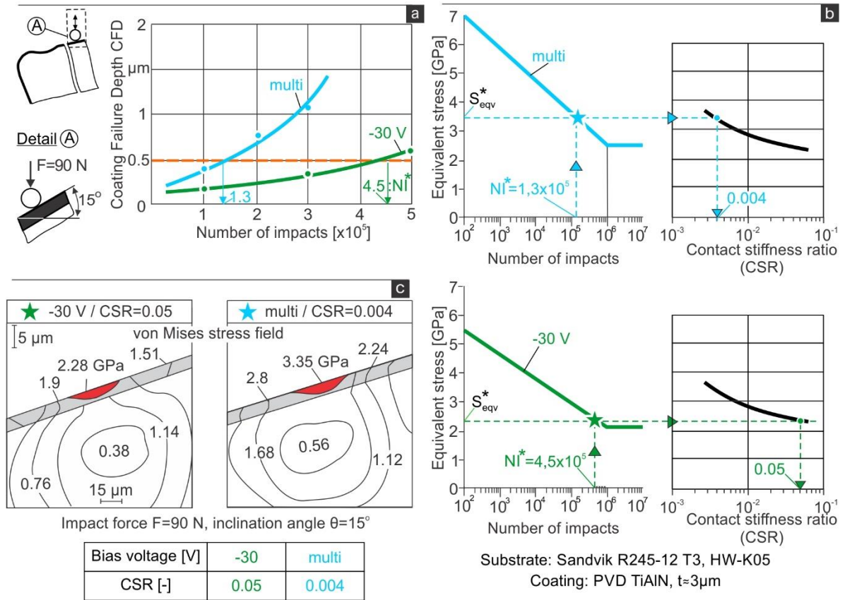
Figure 5. (a) Coating failure depth versus the number of impacts during the inclined impact tests on the investigated PVD films. (b) Determination of the contact stiffness ratios (CSR) quantifying the adhesion of the tested coatings. (c) FEM calculated equivalent stress distributions during the inclined impact test on the prepared coatings at -30 V and multi-bias voltage possessing different adhesion strengths.
