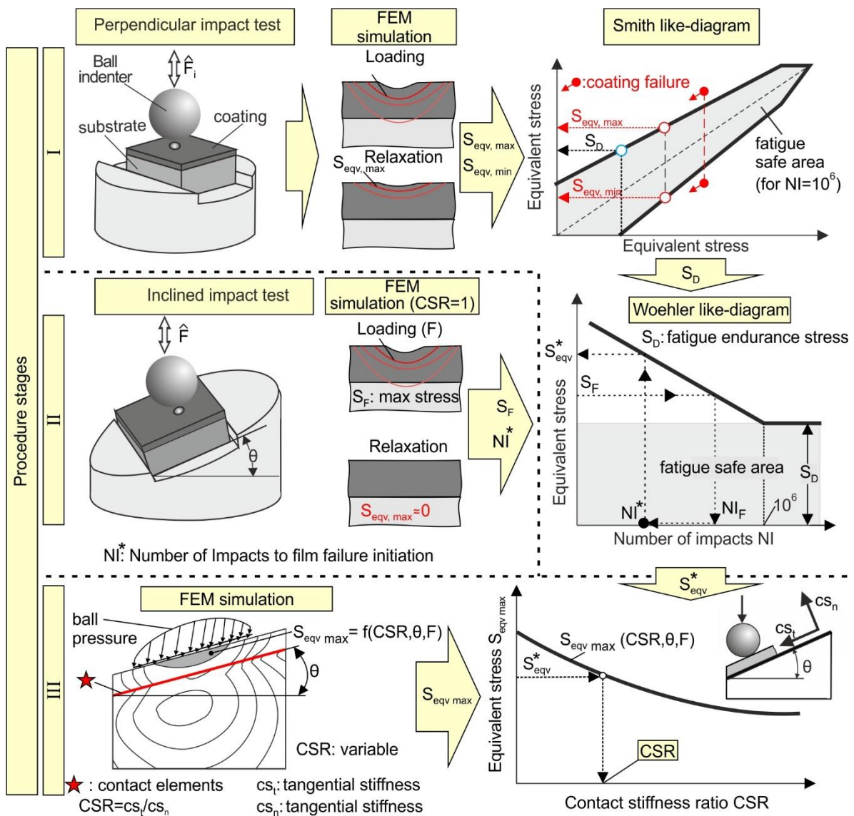
Figure 2. Experimental-computational procedures to determine the fatigue strength and the contact stiffness ratio (CSR) between coating and substrate.
