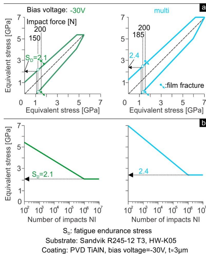
Figure 4. (a) Created Smith-like diagrams of the applied coatings deposited at various bias voltages based on a FEM-supported determination of the developed film stresses during the loading and relaxation stage of the perpendicular impact test. (b) Established Woehler-like diagrams and the defined fatigue endurance stresses of the investigated coatings.
