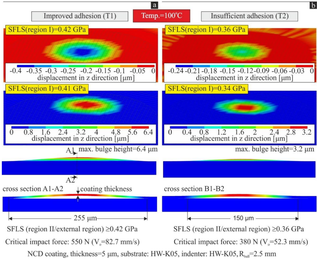
Figure 7. Characteristic NCD coated specimen’s imprints at various SFLSs, after the ball removal at a test temperature of 100°C in the case of improved (a) and insufficient (b) adhesion.
