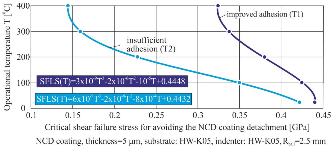
Figure 8. Effect of the operational temperature during inclined impact test on the critical SFLS for avoiding the interfacial fatigue damage of NCD coatings in the investigated adhesion cases.
