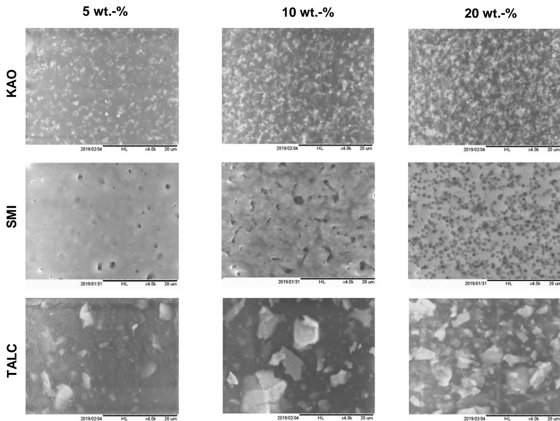
Figure 4. SEM evaluation of natural rubber coatings on paper with different filler types and concentrations (magnification \times 4000 for all images).
