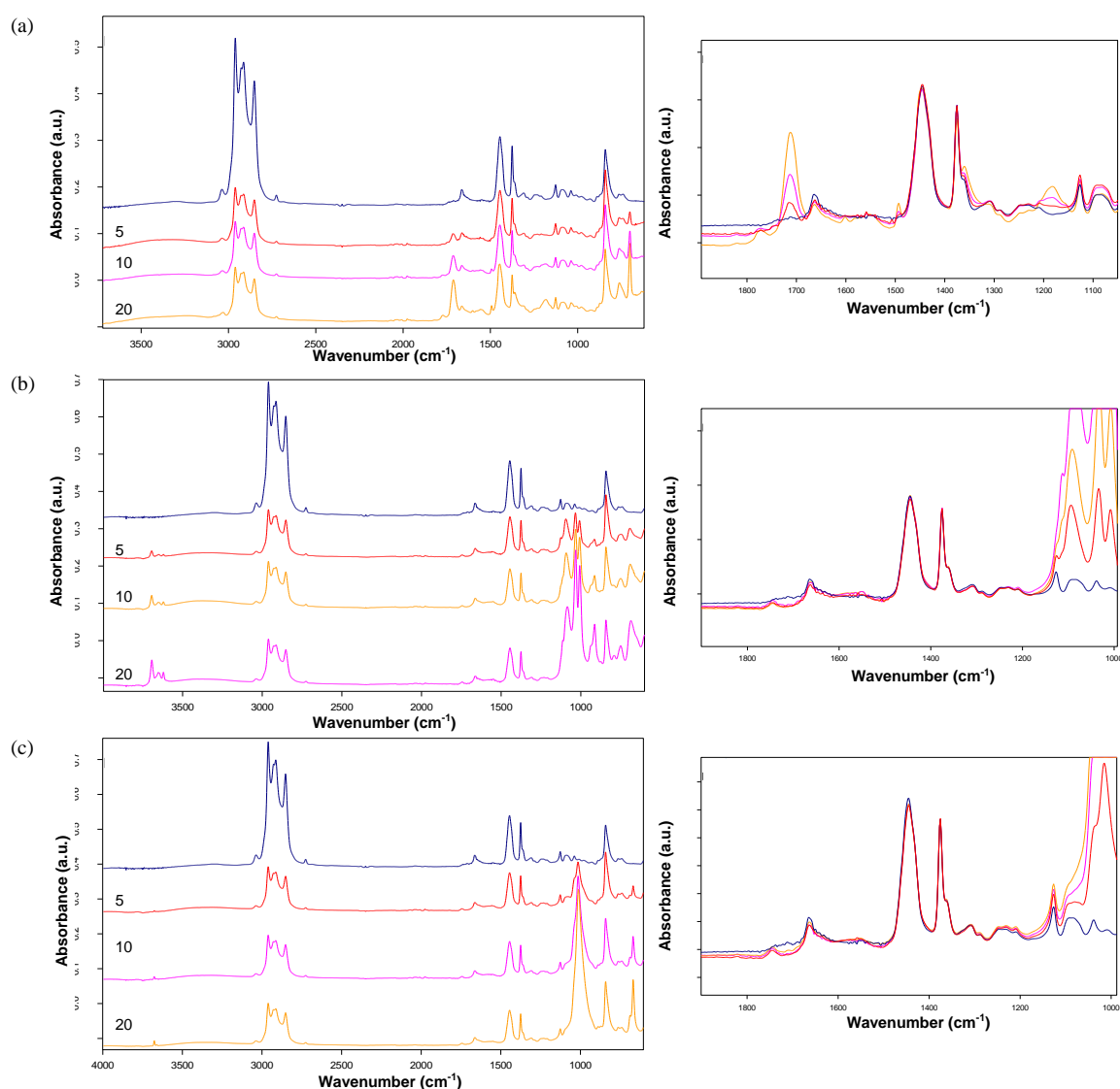
Figure 3. FTIR spectra of natural rubber composites with different concentrations of fillers, (a) SMI nanoparticles, (b) Kaolinite, (c) Talc (same color legend for overview spectra and details at the right).
