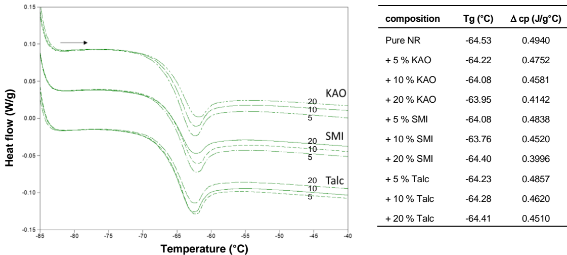
Figure 2. DSC results of natural rubbers with a detail on the glass transition in presence of different types and concentrations of fillers, listing glass transition temperature T_g and heat capacity change \Delta C_p (compositions in wt.-%).
