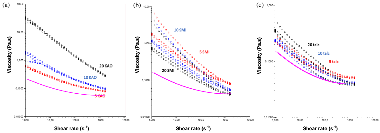
Figure 1. Rheological properties of natural rubber suspensions with different fillers at different concentrations relatively to the unfilled natural rubber suspension (purple curve), (a) Kaolinite, (b) SMI nanoparticles, (c) Talc.
