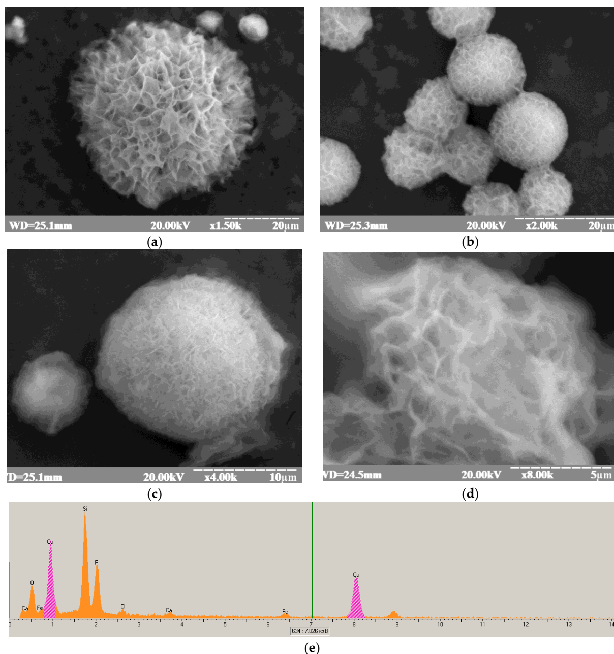
Figure 6. Characteristics of gCuHCFs: SEM images at magnifications of \times 1500 (a), \times 2000 (b), \times 4000 (c) and \times 8000 (d) and X-ray spectral characteristics of gHCFs (e).
