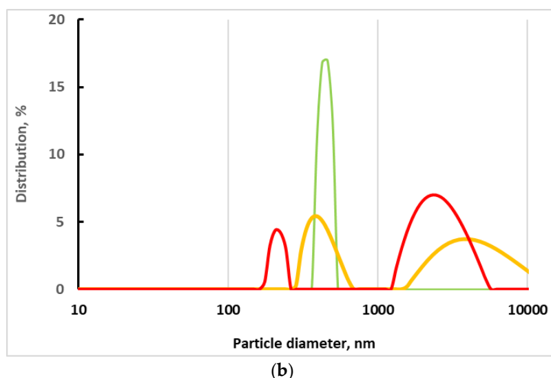
Figure 5. Characterization the gCuHCF: (a)—FTIR spectrum; (b)—DLS plots of particle hydrodynamic diameter of the sample at various concentrations: the green line represents 1.3 \times 10^8 \text{mL}^{-1} , yellow line 6.6 \times 10^7 \text{mL}^{-1} and the red line 3.3 \times 10^7 \text{mL}^{-1} particle concentration.
