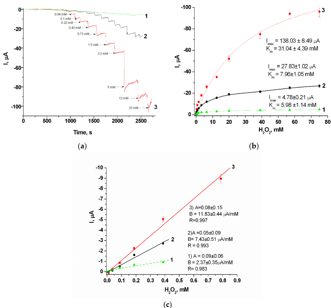
Figure 2. Amperometric characteristics of the modified electrodes: chronoamperograms (a), dependence of the response on increasing concentrations of H 2 O 2 (b) and calibration graphs (c) for PO/GE (1), gFeHCF/GE (2) and gCuHCF/GE (3). Conditions: working potential -50 mV vs. Ag/AgCl (reference electrode), 50 mM NaOAc buffer, pH 4.5 at 23 °C.
