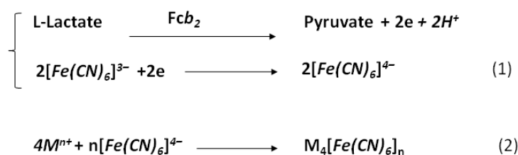
Figure 1. Scheme of gHCF synthesis using Fcb 2 due to enzymatic (1) and chemical (2) reactions; M – transition metal.
