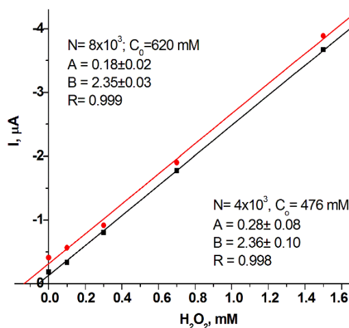
Figure 3. Analysis of a real sample of disinfectant using gCuHCF/GE with the SAT method. Red and black lines correspond to analytes diluted 8,000 and 4,000 times, respectively. H 2 O 2 aliquots were added to the diluted sample up to final concentrations of 0.1, 0.3, 0.7 and 1.5 mM. Conditions: working potential -50 mV vs. Ag/AgCl (reference electrode), 50 mM NaOAc buffer, pH 4.5 at 23 °C.
