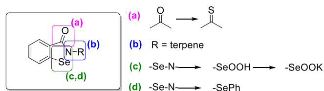
Scheme 1. Structural modification of N -substituted benzisoselenazol-3(2H)-ones.
