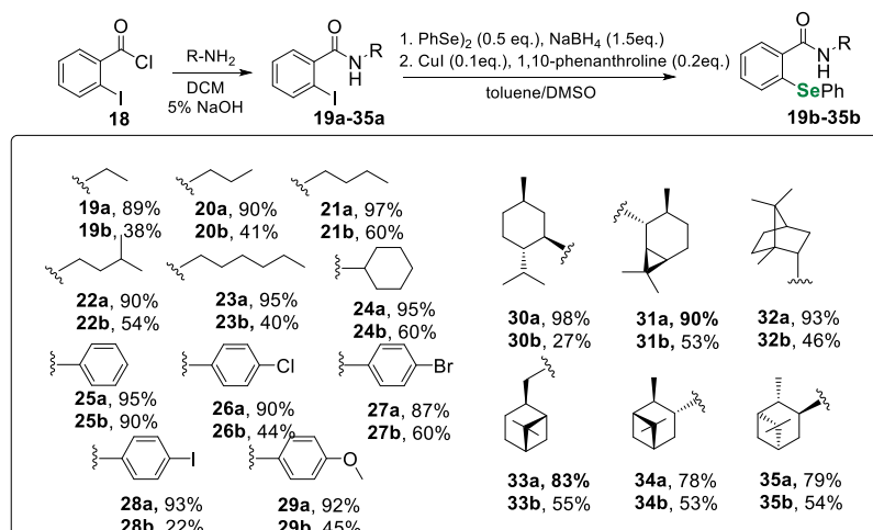
Scheme 5. Synthesis of N-substituted phenylselenides 19b-35b .
