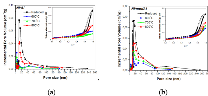
Figure 1. Pore size distribution and N_2 adsorption-desorption isotherms (inset) of the reduced and spent catalysts at 600, 700 and 800°C.
