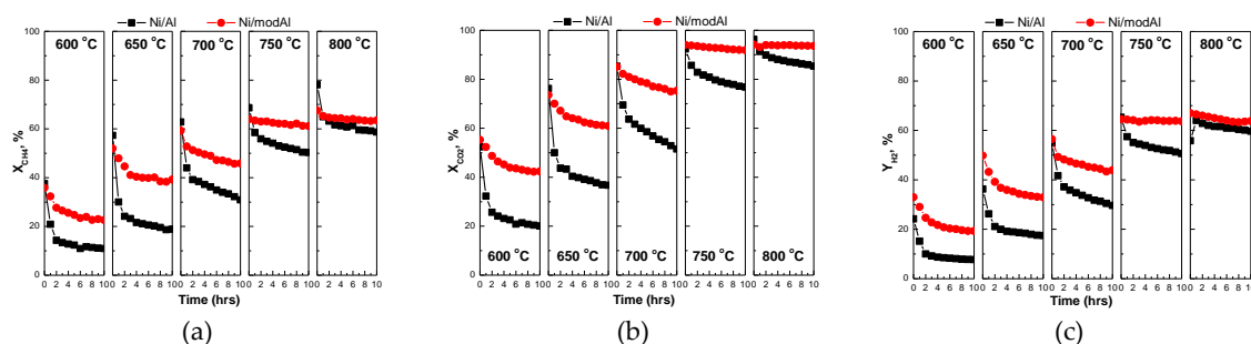
Figure 3. CH 4 and CO 2 conversion (%) for the Ni/Al and Ni/modAl catalysts for stability tests conducted at different temperatures.
