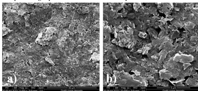
Figure 1. SEM-micrographs of the 'as deposited' coating after spraying Graphit33 lacquer on LDPE.
