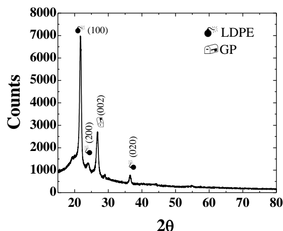
Figure 2. XRD diffractogram of GP film on LDPE.
