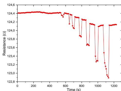
Figure 5. Resistance variation when a pressure is applied and released repeatedly over time.
