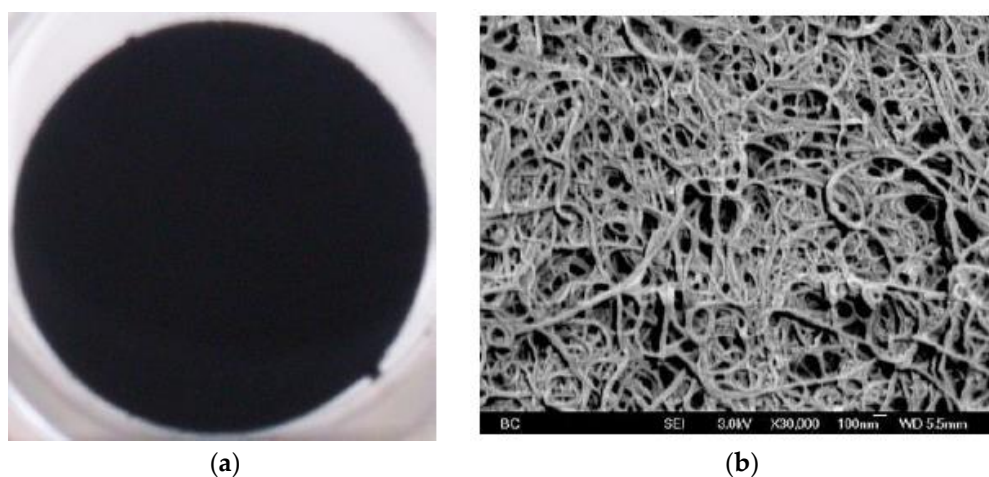
Figure 1. Buckypaper film. (a) Photo of MWNT buckypaper; (b) Typical scanning electron microscope (SEM) image of buckypaper.
