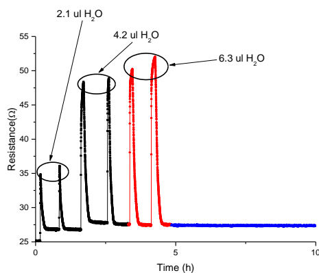
Figure 6. Resistance of the buckypaper when different volumes of water are poured on it.
