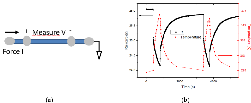
Figure 3. (a) Schematic of the sample used for four-probe electrical measurement. The current is forced in the external probes, and the voltage is measured between the inner ones. (b) Temperature and resistance as function of time.
