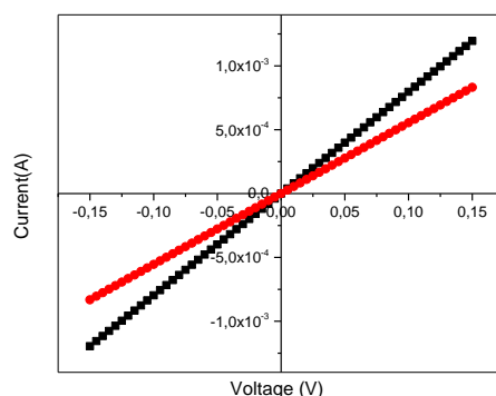
Figure 2. Current-Voltage (I–V) characteristics of the buckypaper measured in four (black line) and two-probe (red line) configurations.
