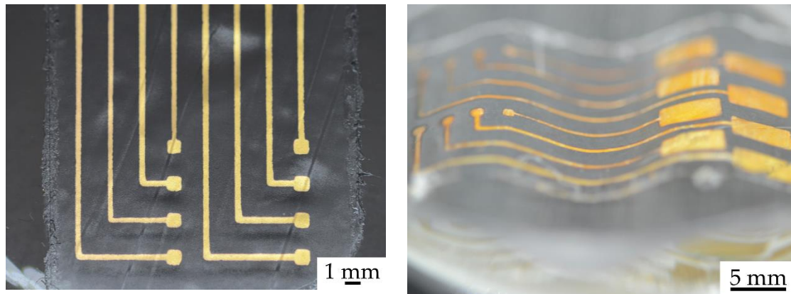
Figure 5. Manufactured ECoG demonstrator with eight electrode contacts (left) and electrode adapted to a wavy shape in PDMS (right).
