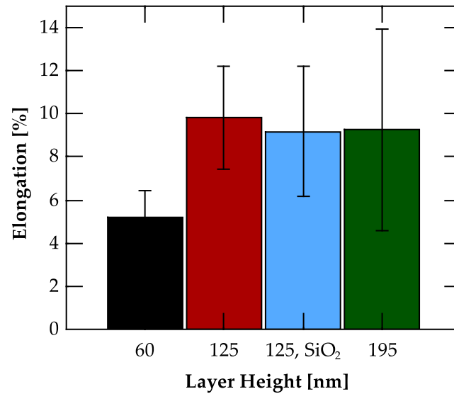
Figure 3. Elongation while maintaining conductivity as a function of the layer height and the performed silicization.
