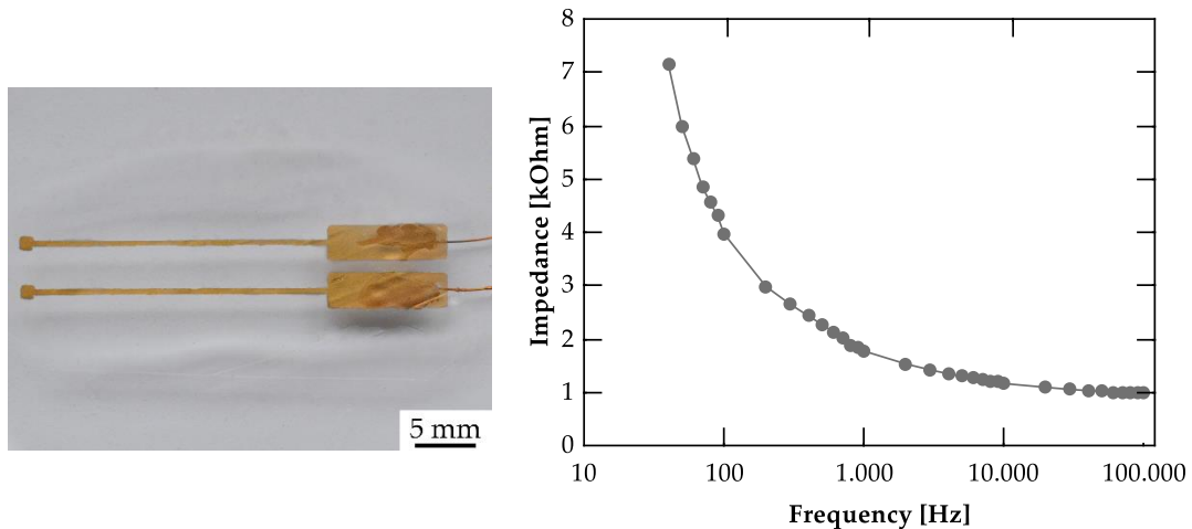
Figure 4. The left illustration shows the setup consisting of two electrode contacts. The right figure shows the measured impedances as a function of frequency.
