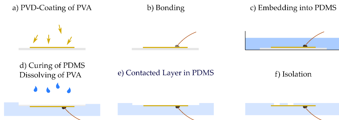
Figure 1. Fabrication process: PVD coating of the transfer substrate (a), contacting (b), embedding in PDMS (c), curing the PDMS and dissolution of the transfer substrate (d) contacted, conductive structure in PDMS (e), insulation (f).
