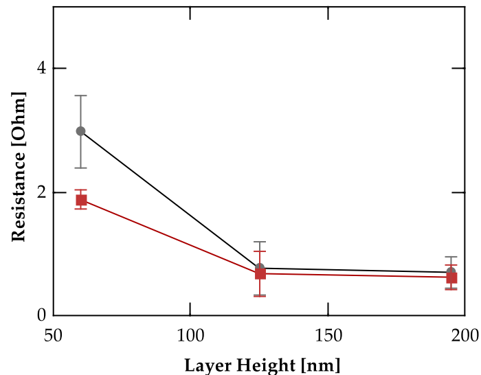
Figure 2. Resistivity as a function of film thickness, before (grey) and after (red) transfer to PDMS.
