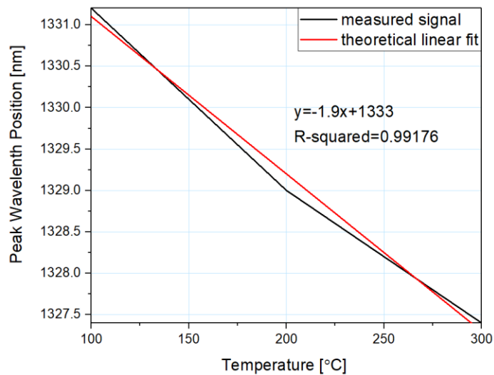
Figure 4. Dependence of the spectral shift of a reflected signal on the temperature.
