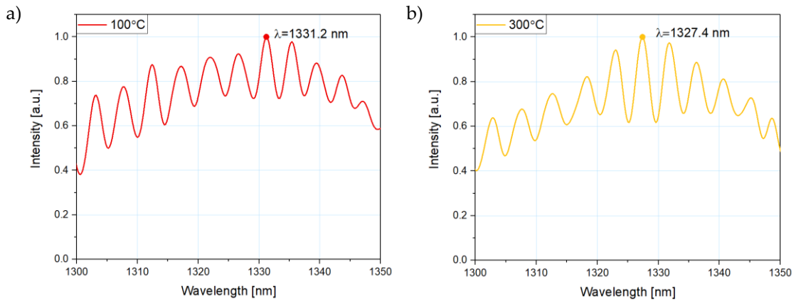
Figure 3. Normalized measured response of the reflected signal for the microsphere-based sensor with 100 nm ZnO ALD coating at: a) 100°C and b) 300°C.
