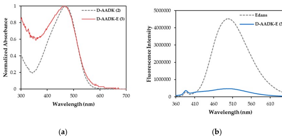
Figure 1. UV/Vis absorption and fluorescence spectroscopy: (a) normalized UV/Vis spectra of peptides 2–3 ( 1 \times 10^{-5} M) at pH 7.5 in phosphate buffer; (b) fluorescence spectra of free Edans and peptide probe 3 ( 1 \times 10^{-5} M) at pH 7.5 in phosphate buffer, upon excitation at 432 nm.
