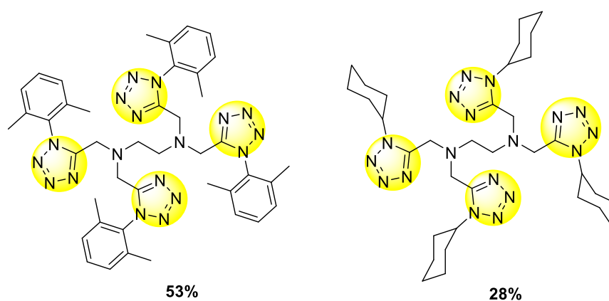
Scheme 2. Substrate scope.
