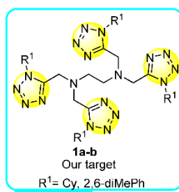
Figure 1. Target compounds.
