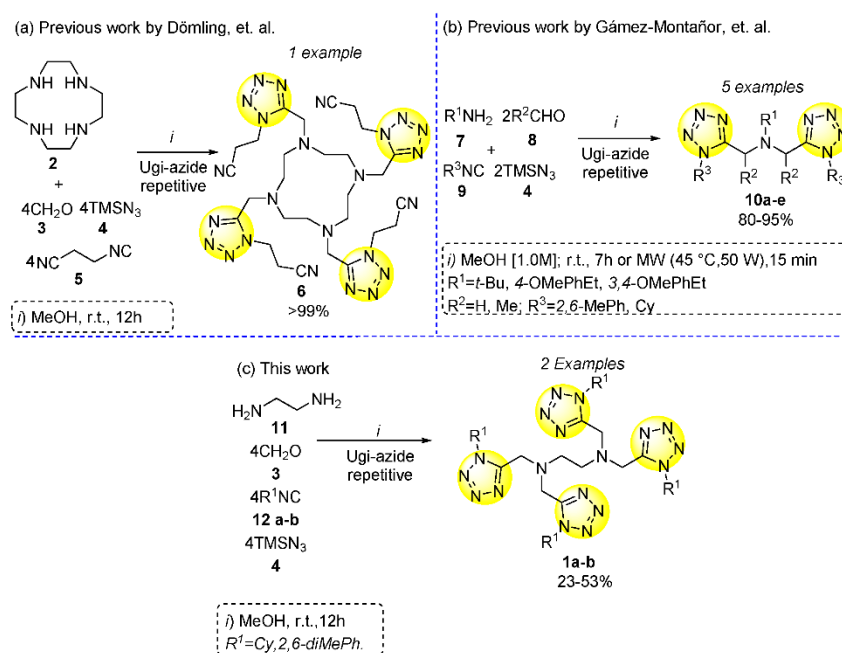
Scheme 1. Previous work and Our work. (a) Previous work by Dömling, et. al.; (b) Previous work by Gámez-Montañor, et. al.; (c) This work.
