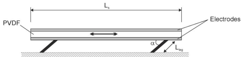
Figure 2. Schematic diagram of the device design. The device consists in a PVDF piezoelectric film metalized at both sides. Two pairs of 3D-printed legs were manually attached to the bottom side of the PVDF film.
