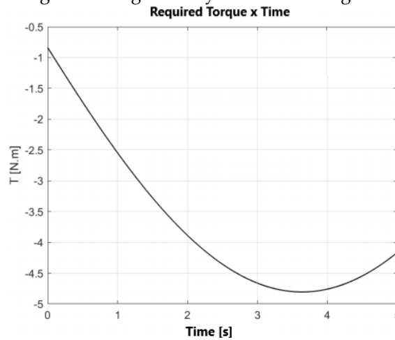
Figure 6. Variation of the required torque to flex the elbow over time.
