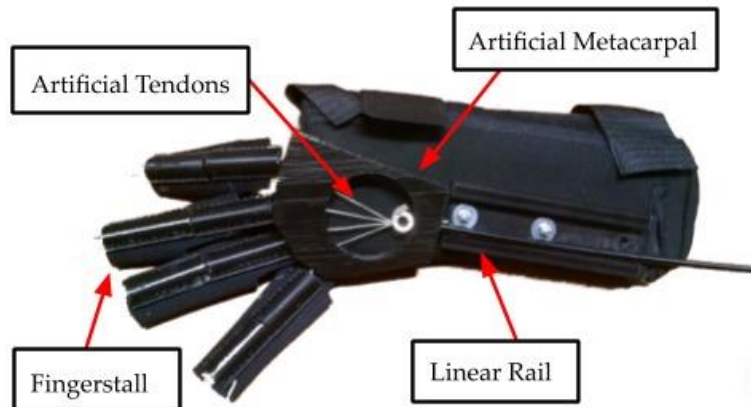
Figure 3. Hand module
