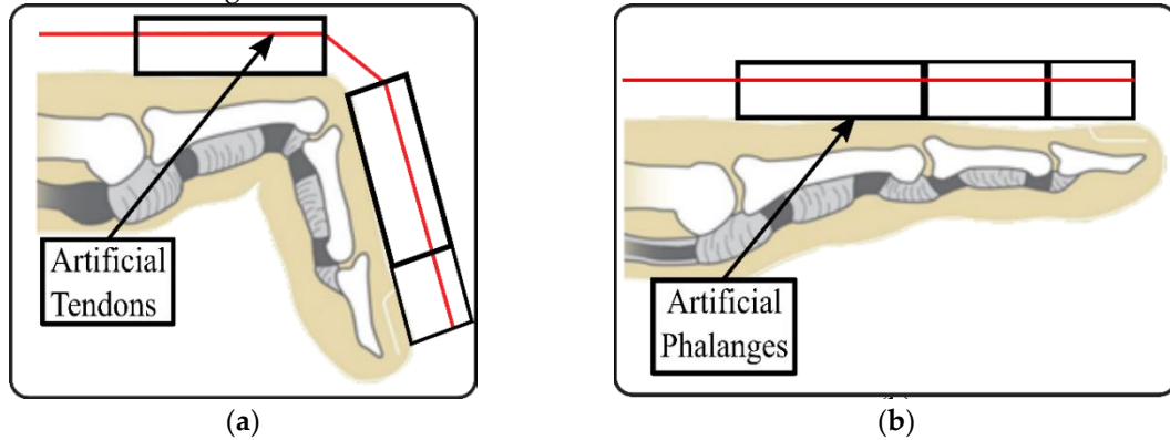
Figure 2. Schematic mechanism representation of (a) closing and (b) opening fingers with artificial phalanx and tendons. Adapted from Rúbio et al. [22]
